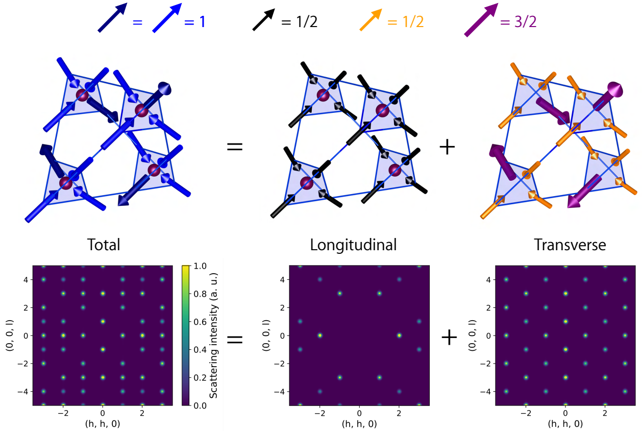
FIG. 7. Top: fragmentation of the spin- R phase magnetic structure - a monopole crystal with ordered transverse fragment. Only half of the tetrahedra are pictured for clarity. Left panel, spin configuration. The minority spins are indicated by a darker shade of blue. Middle, longitudinal fragment \vec{M}_m showing “all spins in all spins out” ordering. Right panel, transverse fragment \vec{M}_d corresponding to the emergent field for the ordered dimer phase (the R -phase, see Fig. (8) top). The colours illustrate the amplitude of each spin component. Bottom: unpolarized neutron scattering intensities in the [hh0] , [00l] plane computed from the corresponding fragment above. The total scattering picture can also be computed by adding the separate intensities of the two fragments.
