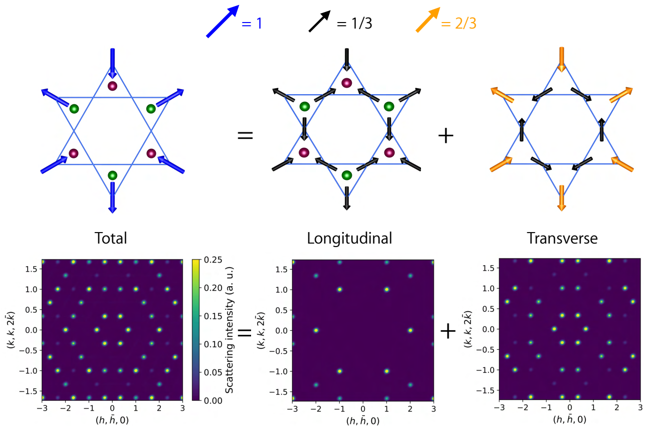
FIG. 4. Top: Fragmentation of the spin- P phase magnetic structure on a kagomé plane. The magnetic unit cell extends over 9 sites. Colours illustrate the amplitude of each component, and green and purple spheres show the placement of positive and negative magnetic charges within the dumbbell model. Left panel, full spin configuration. The quantum resonance on the hexagonal loop results in the effective absence of spins around the loop. Middle panel, longitudinal fragment \vec{M}_m showing “all spins in all spins out” ordering. Right panel, residual transverse fragment \vec{M}_d corresponding to the residual emergent field of the dimer plaquette phase (see Fig. 5 top). Bottom: SF neutron scattering intensities for neutrons polarised perpendicular to the plane computed from the total and corresponding fragment above. The total scattering picture can be computed by adding the separate intensities of the two fragments. Note that the absolute intensity scale is one quarter of that in Fig (3).
