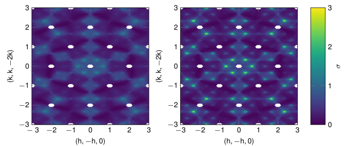
FIG. 6. Unpolarized neutron scattering data in the kagomé plane from Quantum Monte Carlo simulations of quantum nearest neighbour spin ice in a [111] field. Left panel \frac{T}{J} = \frac{1}{20} , right panel \frac{T}{J} = \frac{1}{320} . Data reproduced with permission from [25].
