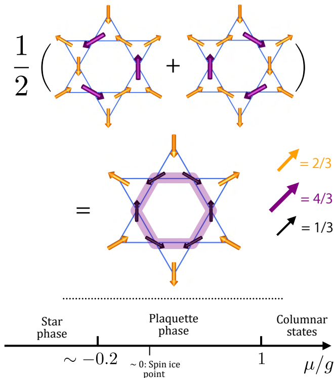
FIG. 5. Top: the quantum resonance of the emergent field for dimers in the plaquette phase is modelled as the average of left and right circulations. Emergent dimers are located on the purple minority spins. The resultant quantum superposition is shown below, with a purple shade illustrating the dimer resonance of the plaquette phase. Colours illustrate the amplitude of each spin component. Bottom: phase diagram of the dimer model given by eqn. (13) on the honeycomb lattice [47].
