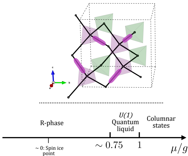
FIG. 8. Top: R -phase dimer structure on the diamond lattice. The tetrahedra shown in Fig. (7) for the spin- R structure are shaded in mauve. The dimer representation is equivalent to the emergent field representation shown in the top right panel of Fig. (7). Bottom: phase diagram [52] for dimers on a diamond lattice as a function of the ratio \mu/g from eqn. (13). Also shown is the “spin ice” point corresponding to the location of the monopole crystal plus small transverse quantum spin fluctuations [53], deep within the spin- R phase.
