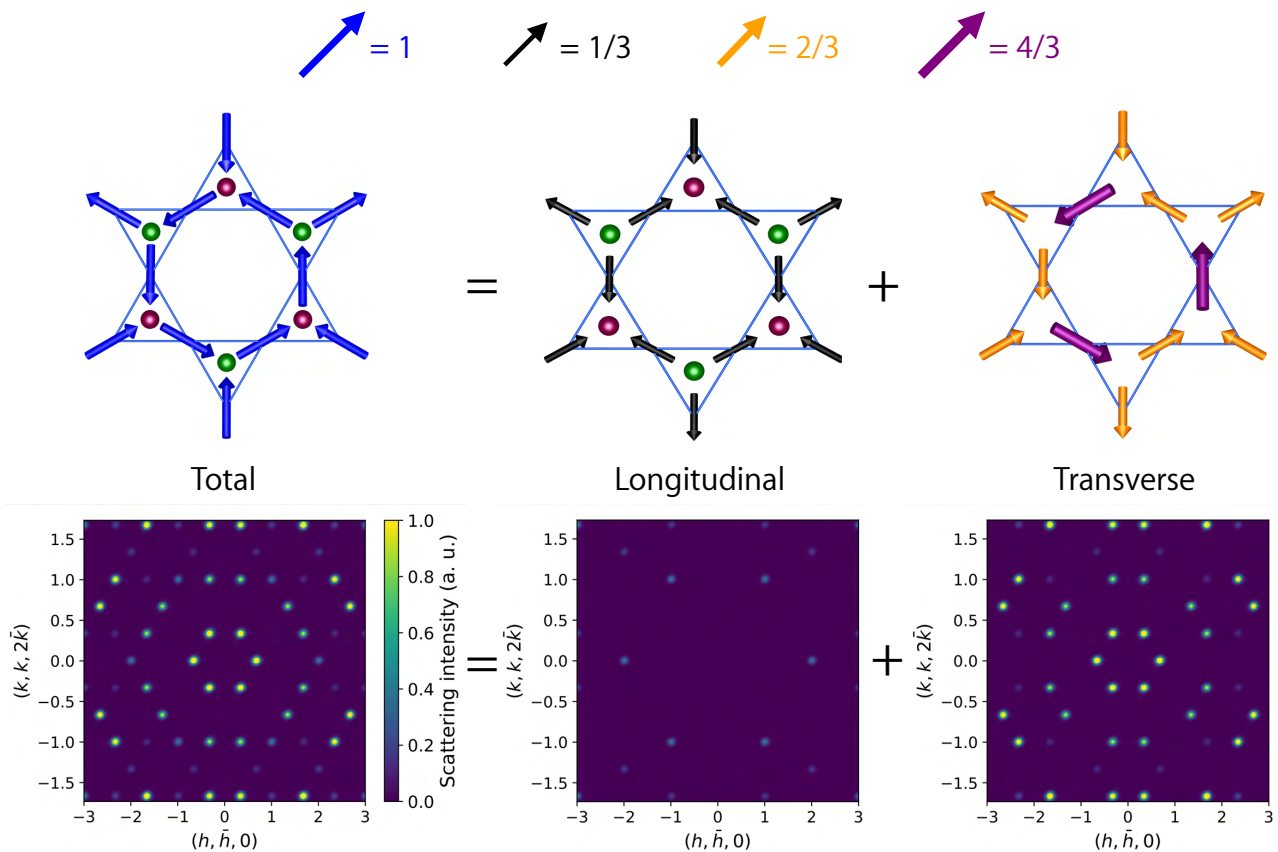
FIG. 3. Top: Fragmentation of the \sqrt{3} \times \sqrt{3} phase magnetic structure on a kagomé plane. The magnetic unit cell extends over 9 sites. Colours illustrate the amplitude of each component, and green and purple spheres show the placement of positive and negative magnetic charges within the dumbbell model. Left panel, full spin configuration. Middle panel, longitudinal fragment \vec{M}_m showing “all spins in all spin out” ordering. Right panel, transverse fragment \vec{M}_d showing emergent ordering of the star phase. Bottom: SF neutron scattering intensities for neutrons polarised perpendicular to the plane computed from the total and corresponding fragment above. The total scattering picture can also be computed by adding the separate intensities of the two fragments.
