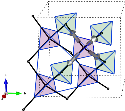
FIG. 1. Pyrochlore lattice (blue) and its dual diamond lattice (black). Tetrahedra of type A ( B ) are shown in shaded purple (green) respectively. The cubic unit cell is delimited by the dashed lines and contains sixteen sites. The grey arrows show the four \vec{d}_i vectors defined in the text.
