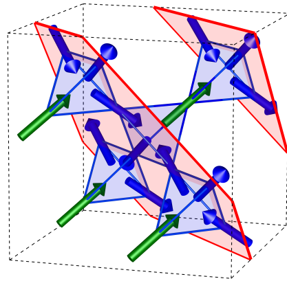
FIG. 2. Pyrochlore spin ice in a [111] field, showing the distinction between planes of pinned apical spins on a triangular lattice (green) and kagome planes satisfying the kagome ice rules (red).
