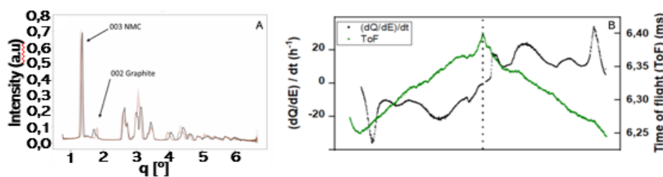
Figure 1. a) X-ray diffractogram acquired on the complete cell; b) Correlation between the electrochemical signal (derived from the galvanostatic curve) and the ultrasound signal
