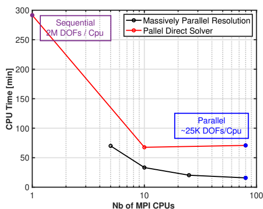
Figure 8: Evolution of the resolution CPU Time with respect to the number of MPI processes.
