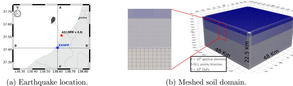
Figure 3: Niigata region with borders of the SEM numerical model at the KKNPP site.
