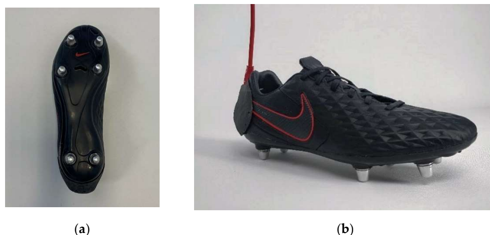
Figure 2. (a) Football shoe with six instrumented studs in the transversal plane (b) and integrated electronics at the back.
