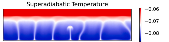
Fig. 13. Snapshot of the superadiabatic temperature in a convection model with a negative Rayleigh number Ra = -10^8 , \mathcal{S} = 5 and r = 1.5 . As show in Fig. 3 convection occurs with these parameters. The colour scale is chosen to emphasize the weak rising plumes and saturates near the surface.
