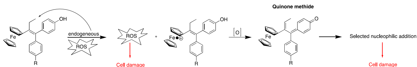
Figure 7. Oxidation sequence of ferrocifens (adapted from [130]).
