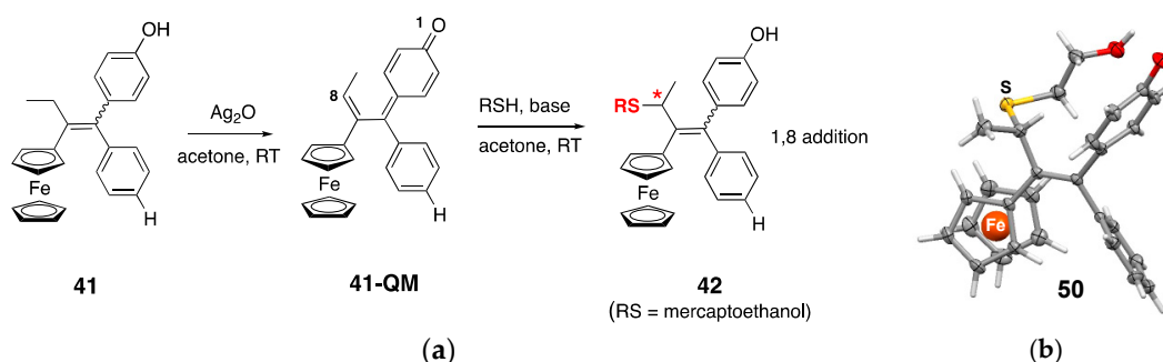
Figure 8. (a) Chemical synthesis of 41-QM followed by 1,8-Michael addition of \beta -mercaptoethanol. * = stereogenic carbon; (b) X-ray structure of the 1,8-adduct with \beta -mercaptoethanol 50 . Adapted from [132].
