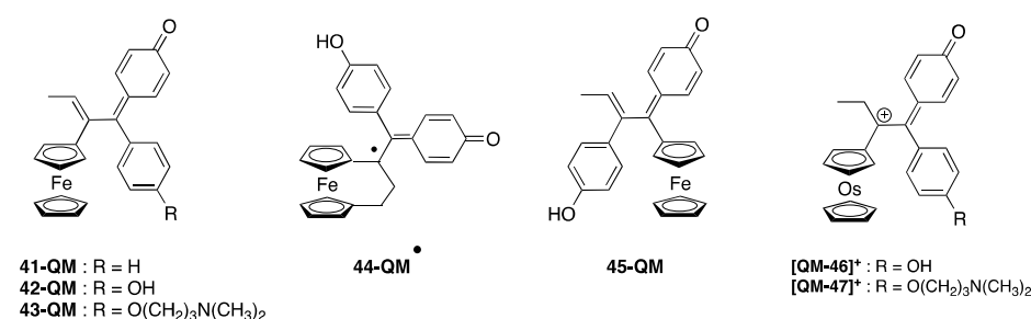
Chart 4. Chemical structure of the complexes obtained by enzymatic oxidation (HRP + H 2 O 2 ) of the complexes depicted in Chart 3.
