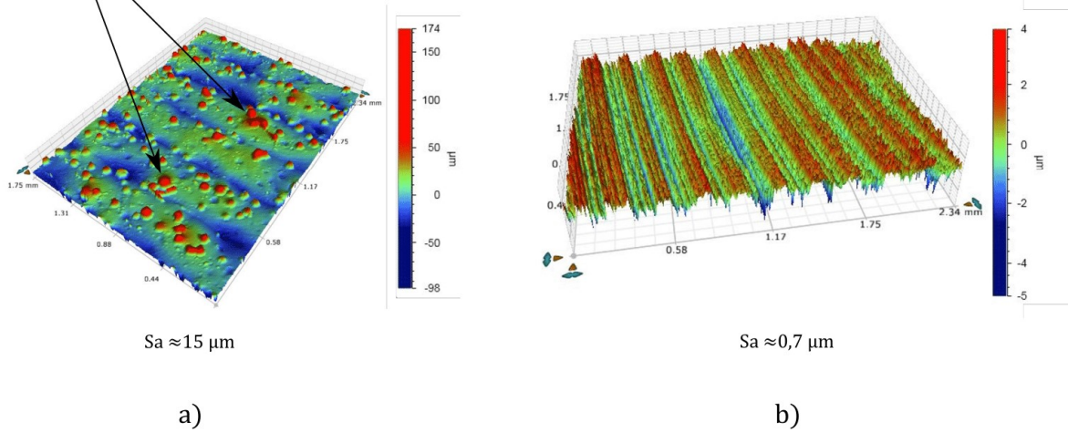
Figure 2: Samples roughness a) before and b) after milling
