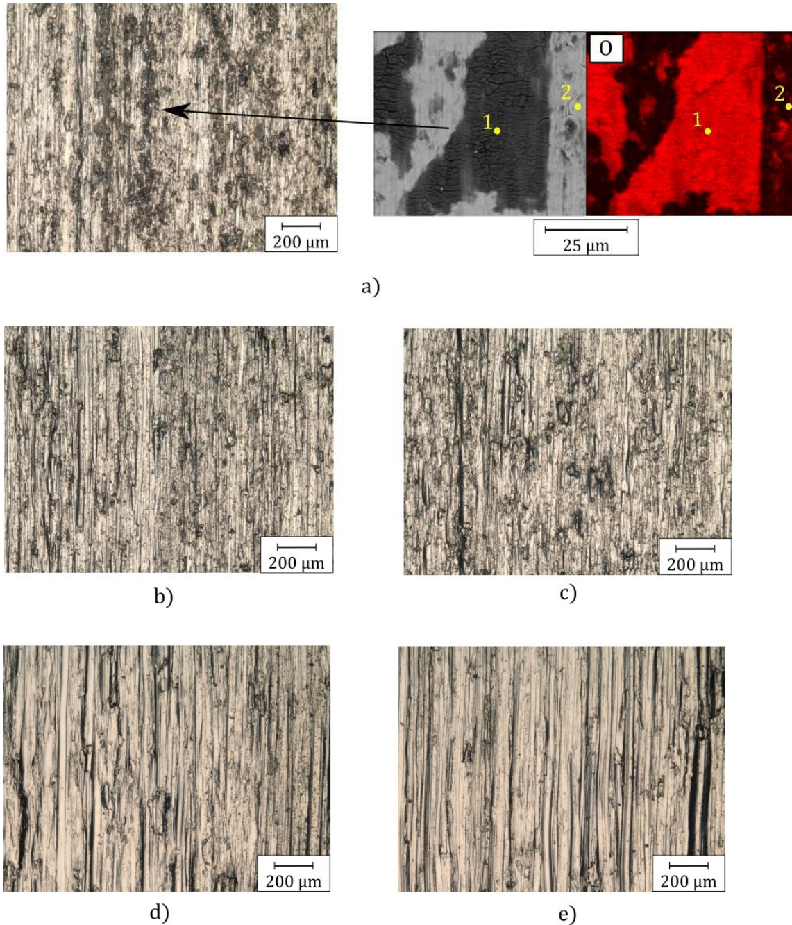
Figure 8: Optical images of worn surfaces of the LMD samples at a) 2 N (with a steady state of the COF); b) 10 N; c) 20 N; d) 40 N; e) 50 N
