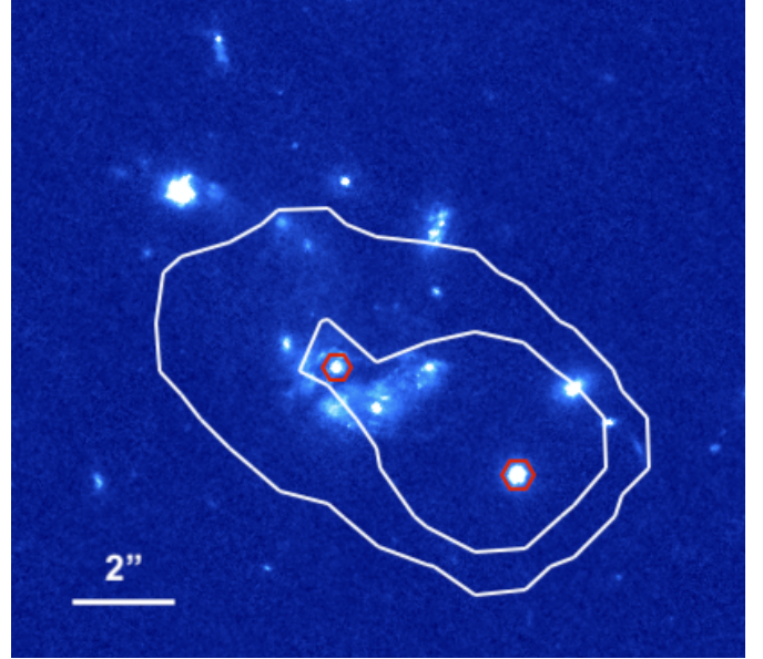
Fig. 10. Chandra 0.5–2 keV X-ray contours (white) overlaid on the NIRCам F115W image. The contours are at 2 \times 10^{-15} ergs s^{-1} cm^{-2} arcmin^{-2} and 2 \times 10^{-14} ergs s^{-1} cm^{-2} arcmin^{-2} (Nandra et al. 2015). The two X-ray AGN are galaxies 89 and 90 (AEGIS 471 and AEGIS 470 respectively), shown by the red polygons.
