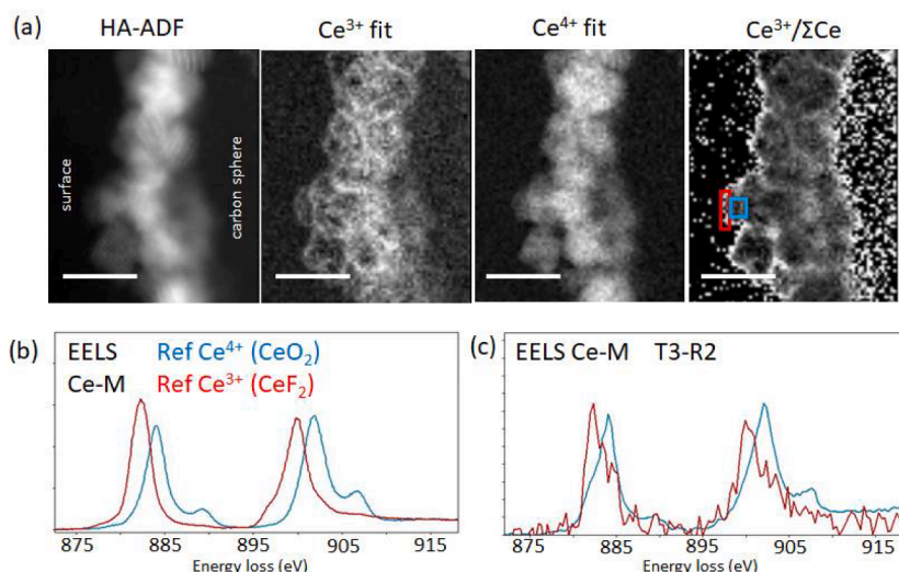
Fig 5. (a) HAADF-STEM, Ce 3+ , Ce 4+ and Ce 3+ /ΣCe maps measured by STEM-EELS experiment for the T3-R2 sample, (b) reference EELS spectra used for a quantification of the Ce 3+ and Ce 4+ contribution, (c) typical EELS Ce-M spectra at the surface of the last particle and at the central part of the last particle (at ca. 2 nm from the surface). The positions of the spectra are indicated by colored boxes in the Ce 3+ /ΣCe map of (a). All scale bars are 10 nm long.
