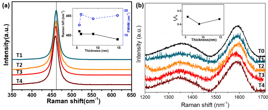
Fig. 3. Raman spectrum of samples T1 to T4. (a) F_{2g} band of the ceria shell. The changes in Raman shift and FWHM of the band with increasing the shell thickness were plotted in the insert figure. (b) D band and G band of the carbon sphere. The ratio between these two bands of samples with different shell thickness was shown in the insert figure.
