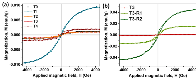
Fig. 4. (a) M-H curves obtained at room temperature of samples T0 to T4. (b) M-H curves of sample T3 and T3 with different reduction treatments.
