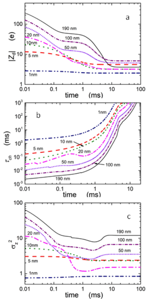
Fig. 1. |Z_d| (a), \tau_{\text{ch}} (b) and \sigma_z^2 (c) as functions of time for P = 0.3 \text{ Torr} , \gamma_m = 0.035 and a_d = 1, 5, 10, 20, 50, 100 , and 190 \text{ nm}
