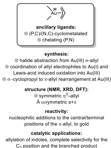
Figure 1. Au(III) \pi -allyl complexes: from their preparation and characterization, to their reactivity and catalytic application.
