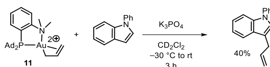
Scheme 5. Stoichiometric reactivity of the (P,N) Au \pi -allyl complex 11 with indole as the nucleophile.
