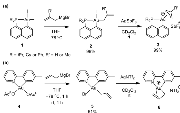
Scheme 1. Preparation of Au(III) \pi -allyl complexes 3 and 6 (OAc F = OCOCF 3 ) upon halide abstraction from \sigma -allyl complexes 2 and 5 . The yields given for complex 2 and 3 are for R = i Pr and R' = H. No yield reported for 6 as it starts to decompose at the same time as it forms.
