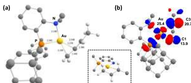
Figure 3. (a) Optimized geometry of the Au(III) \pi -allyl complex (P,N)Au[H 2 CC(H)CH(CH 3 )] 2+ at the SDM(CH 2 Cl 2 )-B3PW91/SDD + f(Au),6-31G** (other atoms) level of theory (distances in Å). Simplified perspective view as inset chart. (b) Plot of the LUMO (cutoff: 0.05) with key atomic contributions in %.
