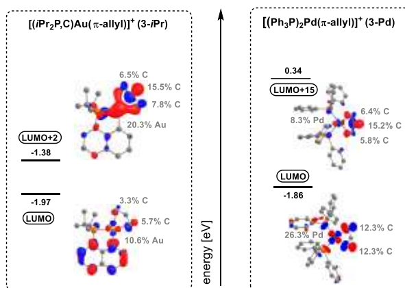
Figure 2. Key Molecular Orbitals (MO) computed for complexes 3-iPr and 3-Pd . Energy of the MOs in eV, cutoff: 0.05. Contribution of the main atoms in each MO in %.
