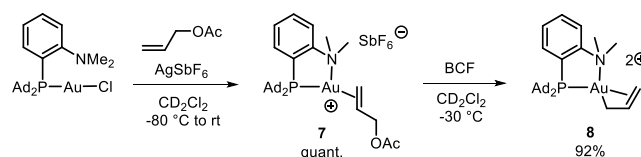
Scheme 2. Formation of the Au(I) \pi -alkene complex 7 and subsequent Lewis acid-assisted oxidation to give the Au(III) \pi -allyl complex 8 . SbF 6 - and AcO-BCF - counter-anions for 8 .
