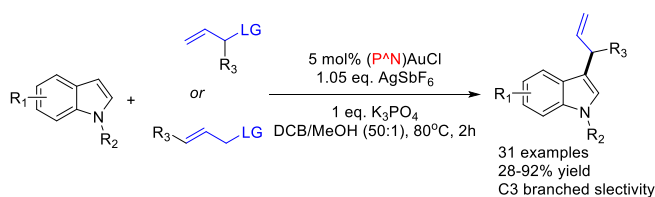
Scheme 6. Ligand-enabled Au(I)/Au(III) catalytic allylation of indoles with allyl electrophiles.
