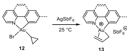
Scheme 2. Formation of the (N,C) Au(III) \pi -allyl complexes 13 from their corresponding Au(III) \sigma -cyclopropyl complexes 12 by halide abstraction.
