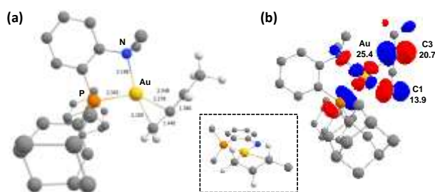
Figure 3. (a) Optimized geometry of the Au(III) \pi -allyl complex (P,N)Au[H 2 CC(H)CH(CH 3 )] 2 2+ at the SDM(CH 2 Cl 2 )-B3PW91/SDD + f(Au),6-31G** (other atoms) level of theory (distances in Å). Simplified perspective view as inset chart. (b) Plot of the LUMO (cutoff: 0.05) with key atomic contributions in %.
