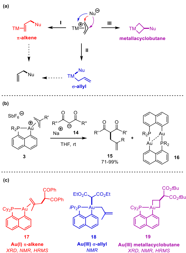
Scheme 3. (a) Possible reactive sites for the nucleophilic addition to transition metal \pi -allyl complexes. (b) Reactivity of complexes 3 ( R = iPr or Cy , R' = H or Me ) towards \beta -diketo enolates 14 ( R'' = OEt , OtBu or Ph ). (c) Examples of characterized complexes ( 17-19 ) showing nucleophilic addition to the central and terminal position of the \pi -allyl, as well as to gold.
