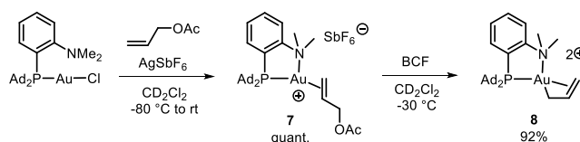
Scheme 2. Formation of the Au(I) \pi -alkene complex 7 and subsequent Lewis acid-assisted oxidation to give the Au(III) \pi -allyl complex 8 . \text{SbF}_6^- and \text{AcO-BCF}^- counter-anions for 8 .
