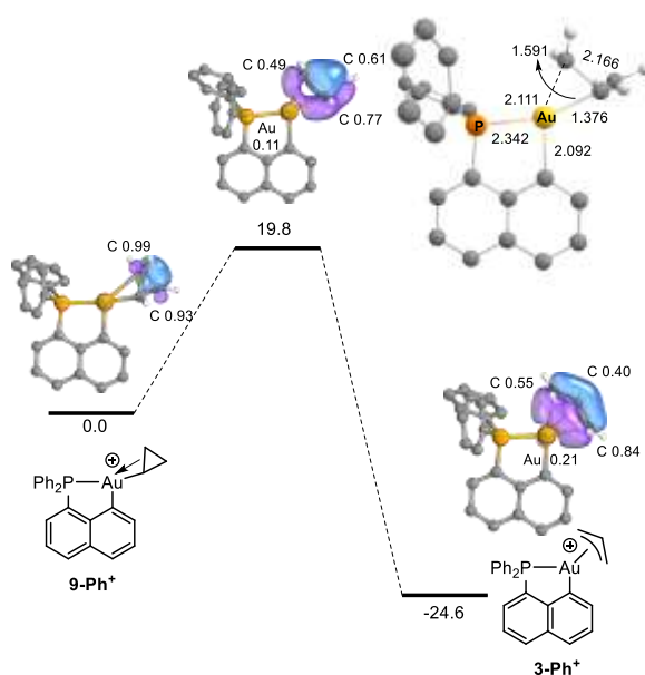
Figure 2. Computed energy profile for the ring-opening of the (P,C) Au(III) \sigma -cyclopropyl complex 9-Ph to give the corresponding \pi -allyl complex 3-Ph . \Delta G values in kcal/mol, main distances in Å. Profile computed in the gas phase at the B3PW91/SDD+f(Au), 6-31G** (other atoms) level of theory. And main IBOs accounting for the ring-opening of the distal \sigma (CC) bond along the reaction path (numbers relate to the fraction of electrons of the doubly occupied orbital assigned to each atom).
