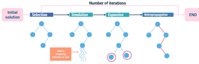
Fig. 1. Steps of the MCTS-CD.
