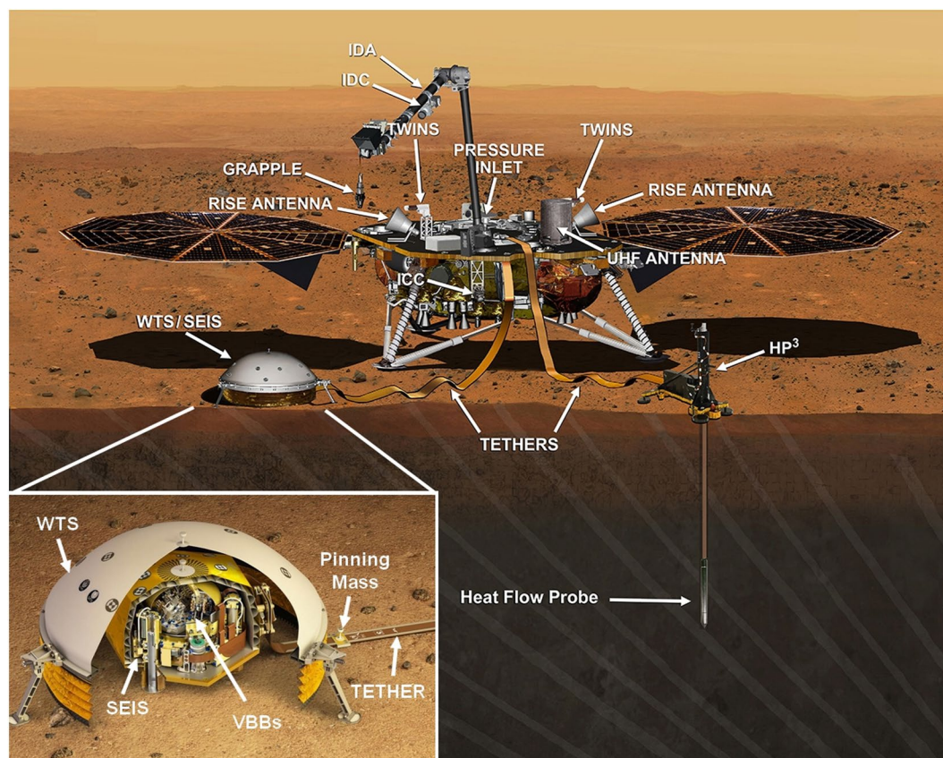
Figure 1. Artist view of the InSight lander and SEIS instrument (credit NASA –InSight mission and IGP D.Ducros).
