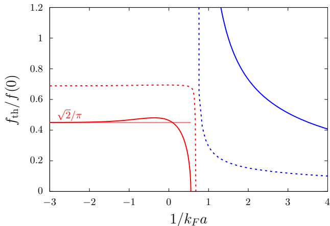
FIG. 2: The spectral weight of the pair-breaking edge f_{\text{th}} (relative to the static response f(0) ) as a function of the interaction strength at T = 0 (solid curves) and T = 0.999T_c (dashed curves). In red the BCS regime where the edge exhibits a squareroot divergence (upper line of Eq. (??)), in blue the BEC regime where instead this edge is a squareroot cancellation (lower line of Eq. (??)). Note that the boundary between those two regimes depends weakly on temperature.
