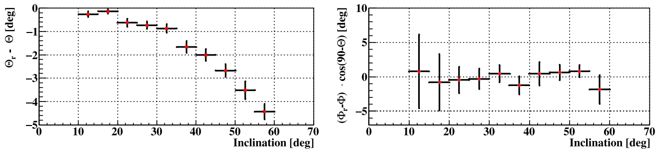
Fig. 34 Mean value and standard deviation of \Delta\Theta = \Theta_{rec} - \Theta_{sim} (left) and \Delta\Phi = (\Phi_{rec} - \Phi_{sim}) \cos(90 - \Theta) (right) plotted against the true zenith angle (inclination) for EUSO-Balloon. Image adapted from [97]
