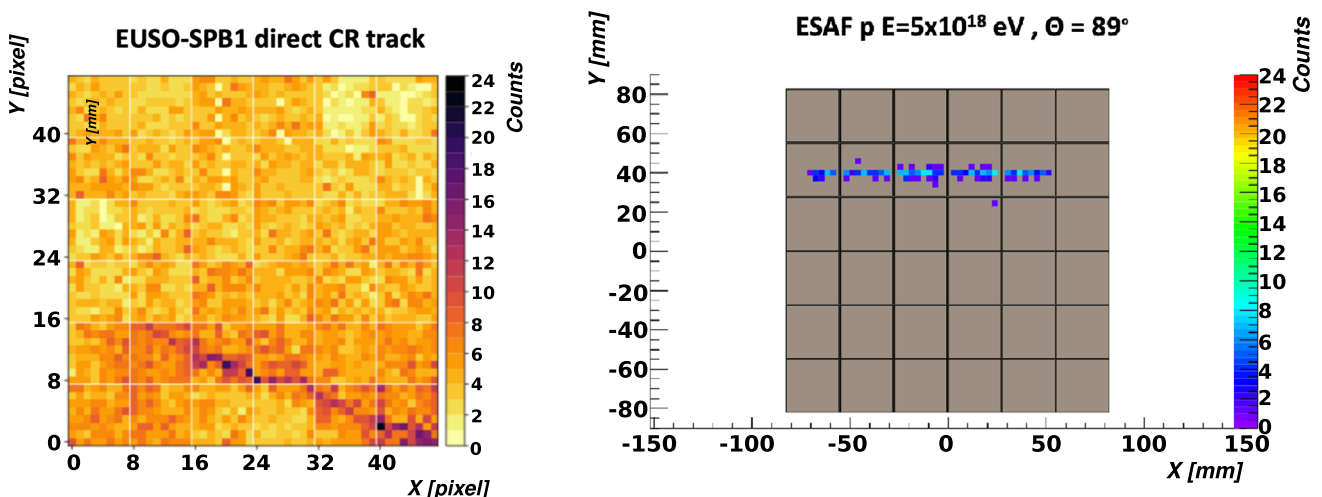
Fig. 32 Left side: Direct cosmic ray triggering the EUSO-SPB1 detector. Right side: Simulated proton EAS of energy E = 5 \times 10^{18} eV crossing the balloon FoV at \sim 25 km altitude with a zenith angle of \theta = 89^\circ . They both correspond to 1 GTU data
