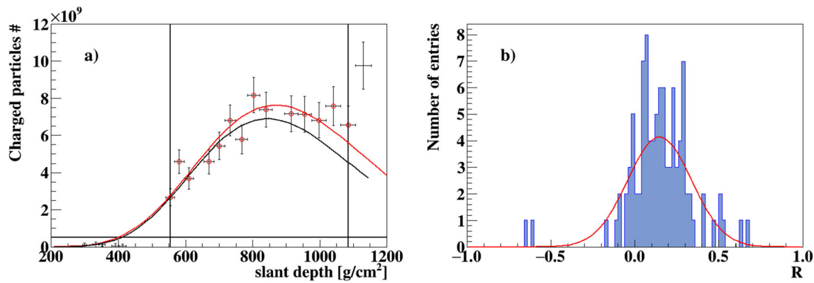
Fig. 33 Panel a: We show here an example of an event reconstructed by EUSO-Balloon. The continuous black line indicates the real simulated shower profile (the number of charged particles in the shower at each slant depth). The black points show the reconstructed profile as obtained by the algorithms. The points which are accepted as fit data are indicated by red circles and the GIL fit applied to these points is shown by the continuous red line. We clearly see how the automatic fit correctly excluded the Cherenkov mark visible at the end of the curve.
