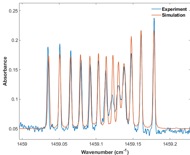
Figure 6: Cluster J' = 42 of the \nu_{15} P-branch
