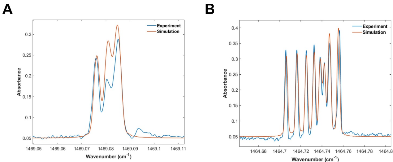
Figure 5: A – Cluster J' = 10 B – Cluster J' = 24
