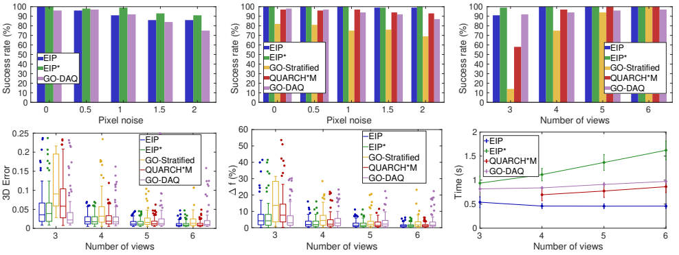
Figure 3: Comparisons with the state of the art. Top: success rate using 3 views (left) and 4 views (middle) with varying noise levels, and using 3-6 views with 1 pixel noise level (right). Bottom: distribution of 3D error (left) and focal length error (middle), and runtime results (right) using 3-6 views with 1 pixel noise level.
