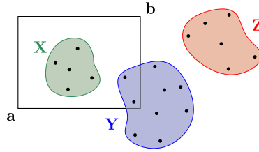
Fig. 4. The collection X is in the interval (\mathbf{a}, \mathbf{b}) , Z is outside (\mathbf{a}, \mathbf{b}) , and (\mathbf{a}, \mathbf{b}) splits Y . Subfamilies \{X, Y\} and \{X\} are all (\mathbf{a}, \mathbf{b}) -proper subfamilies of \{X, Y, Z\} . \{X, Y, Z\} is 1-feasible with respect to (\mathbf{a}, \mathbf{b}) since only Y is split by the interval.
