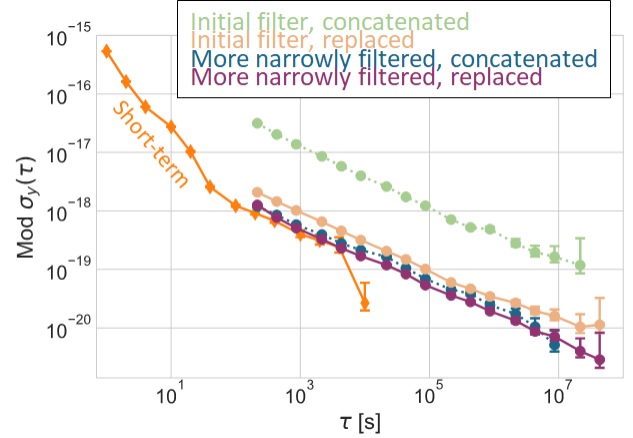
Figure 4: End-to-end stability (modified Allan deviation) for the Paris-Strasbourg-Paris link along 5 years of data. Missing data are taken into account either by concatenating the data or by replacing missing data with simulated data having the same statistical properties.
