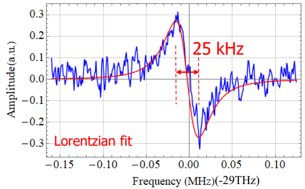
Figure 7: saturated absorption spectrum of the line P(E,co,0,2,33) of methanol at a pressure of 0,05 Pa, around 29 THz (10 \mu\text{m} ), with 1s/point. The signal is detected in transmission of a Fabry-Perot cavity with a Quantum Cascade Laser stabilised to the REFIMEVE signal.
