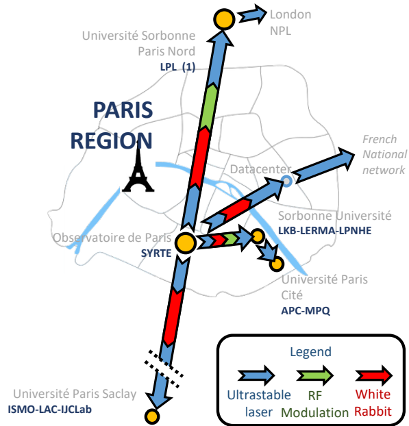
Figure 5: schematic of the REFIMEVE regional network in Paris.
