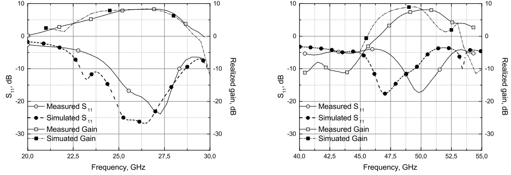
Figure 5: Comparison between measured and simulated realized gain and matching
