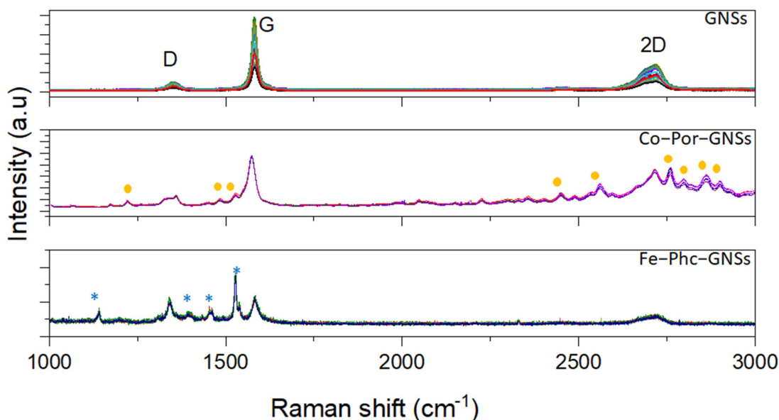
Figure 1. Raman spectra of (top to bottom) solution-processed graphene nanosheets (GNSs), Co-Por-GNSs, and Fe-Phc-GNSs ( \lambda_{exc} = 532 nm).
