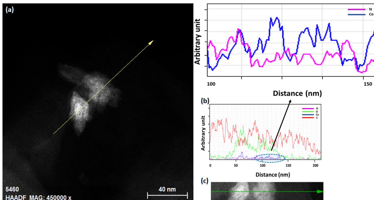
Figure 5. STEM-HAADF-EDS line scan analyses of Co-Por functionalized GNSs: (a) STEM-HAADF micrograph on the chosen area where a line scan along the direction indicated by the yellow arrow was performed. (b) Corresponding STEM-EDS line scan spectrum showing the variation of the Nitrogen (in pink), Cobalt (in blue), Carbon (in red), and oxygen (in green) signal recorded along the scanning direction indicated by the green arrow in (c). (c) Zoom of the analyzed area indicated by the yellow arrow in (a).
