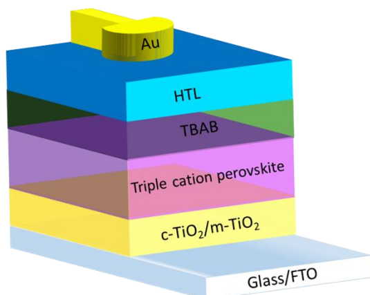
Figure 5. Device structure of the n-i-p PSC (a). Energy level diagram of the components of the n-i-p PSC (b).
