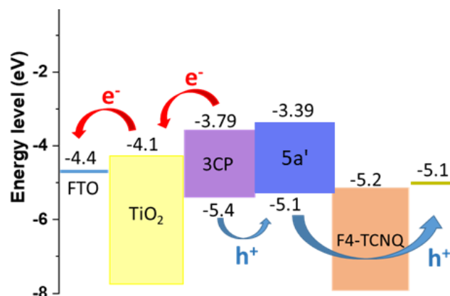
Figure 5. Device structure of the n-i-p PSC (a). Energy level diagram of the components of the n-i-p PSC (b).
