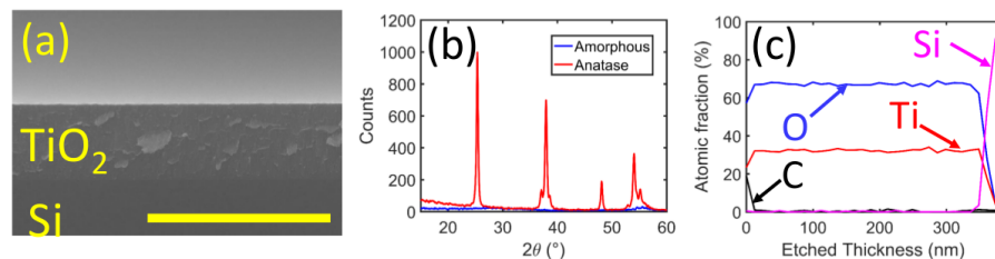
Fig. 1. (a) Scanning Electron Microscope image of an amorphous e-gun deposited amorphous TiO 2 layer on a silicon substrate (scale bar 1 μm). (b) X-Rays Diffraction spectra for amorphous and anatase TiO 2 layers. (c) X-Rays Photoelectron Spectroscopy analysis of an amorphous TiO 2 layer.
