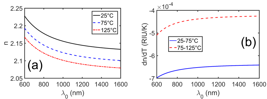
Fig. 2. (a) Dispersion of the purely real refractive index of an amorphous 400 nm-thick amorphous TiO 2 . (b) Thermo-Optic coefficient (TOC) dispersion as a function of the temperature range.
