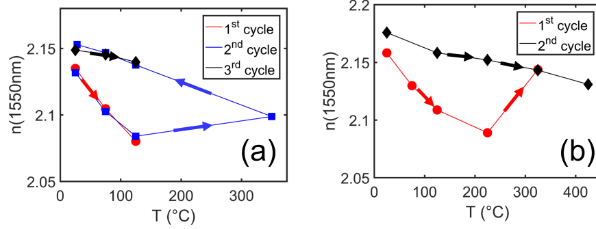
Fig. 3. (a) Temperature dependent refractive index ( \lambda_0 = 1550 nm) of a 435 nm-thick amorphous TiO 2 during subsequent heating cycles. (b) Same as (a) for a 420 nm-thick amorphous TiO 2 layer.
