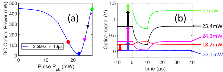
Fig. 8. (A) DC optical signal at the cross port for 2.5kHz pulse with a fixed duration ( 10\mu\text{s} ) and increased peak-power. (b) Optical pulses recorded for increasing peak-powers. For each peak-power, the DC optical signal is displayed in (a) with a dot of same face color as the corresponding optical signal.
