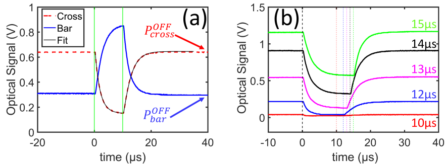
Fig. 7. (a) Comparison of optical cross and bar output signal in case of pulsed TO activation of the MZI at a frequency of 2.5kHz with 10\mu s -long pulses at peak power of 33mW. (b) Monitoring of a MZI cross optical signal for pulses of same peak power but increasing duration.
