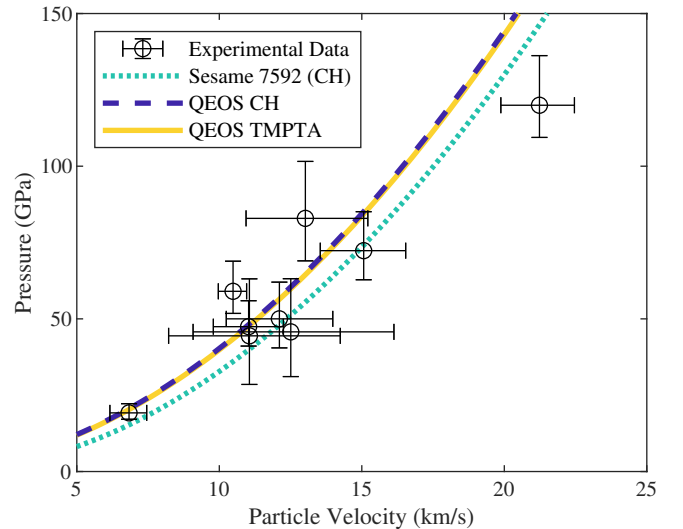
FIG. 8. Experimental Up-P data compared to principal Hugoniots generated from a range of EOS models. The error bars come from a MC analysis of 10,000 random samples (these error bars are symmetric around the mean of the distribution, which is slightly different from the value calculated through the ‘exact’ calculation - leading to the asymmetry).
