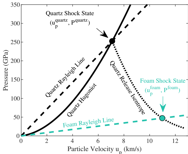
FIG. 4. The impedance matching calculation for the data from Figure 3, shown graphically. The intercept of the known Quartz Hugoniot and the Quartz Rayleigh line (defined by the measured quartz shock velocity) provides the shocked quartz state. This is used to calculate the appropriate quartz release isentrope. The intercept of this with the foam Rayleigh line provides the foam shock state.
