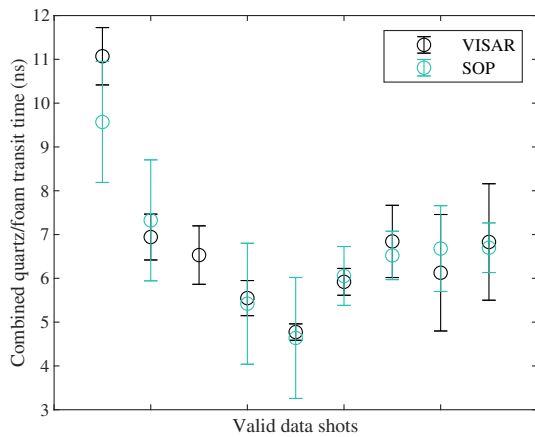
FIG. 7. Combined quartz and foam transit times, as determined for each valid data shot from the VISAR and SOP. All shots agree to within the error (which is due to uncertainty in identifying the relevant behaviours in the raw data, and the finite slit width of the streak cameras).
