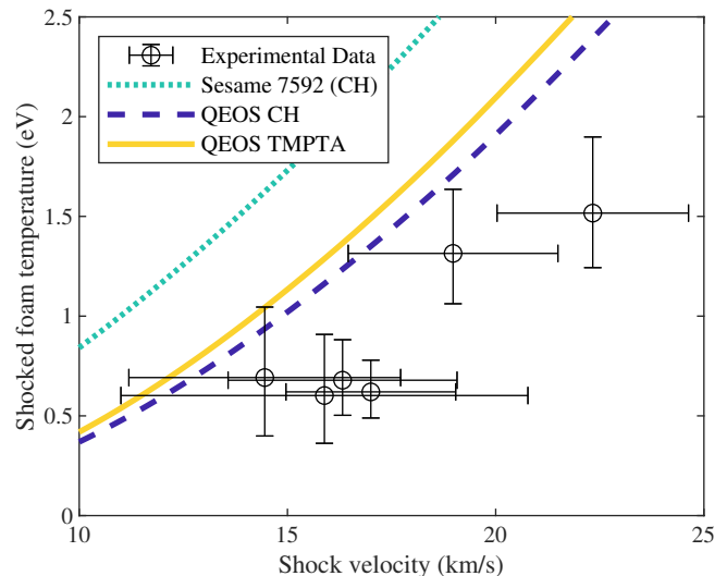
FIG. 10. Grey-body temperature for the shocked foam as a function of shock velocity. Despite the large error bars, the theoretical models are not within the uncertainty of most shots.
