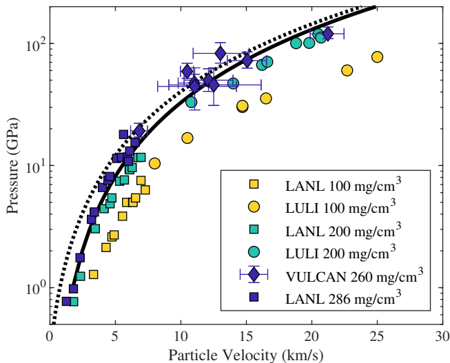
FIG. 9. Up-P experimental data from a series of experiments on low-density foams. The SESAME and QEOS CH hugoniots are displayed as the solid and dashed lines respectively (the TMPTA QEOS overlaps the CH QEOS, and so has been omitted). Error bars are displayed for the VULCAN data (but omitted from other sets due to data availability and visibility). Colour indicates foam density, while shape indicates the source of the data. The NRL data is at higher particle velocity and pressure and so does not appear on these axis, but continues the trend for the 100 mg/cm 3 data.
