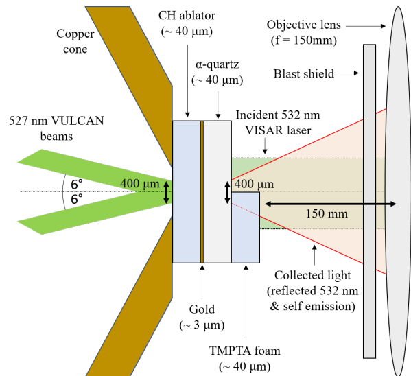
FIG. 2. Simple schematic showing the target and objective lens (top view, not to scale)
