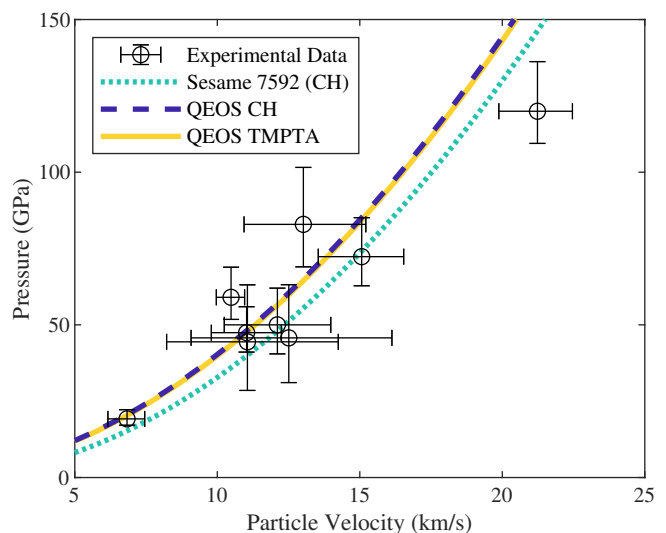
FIG. 8. Experimental Up-P data compared to principal Hugoniots generated from a range of EOS models. The error bars come from a MC analysis of 10,000 random samples (these error bars are symmetric around the mean of the distribution, which is slightly different from the value calculated through the ‘exact’ calculation - leading to the asymmetry).
