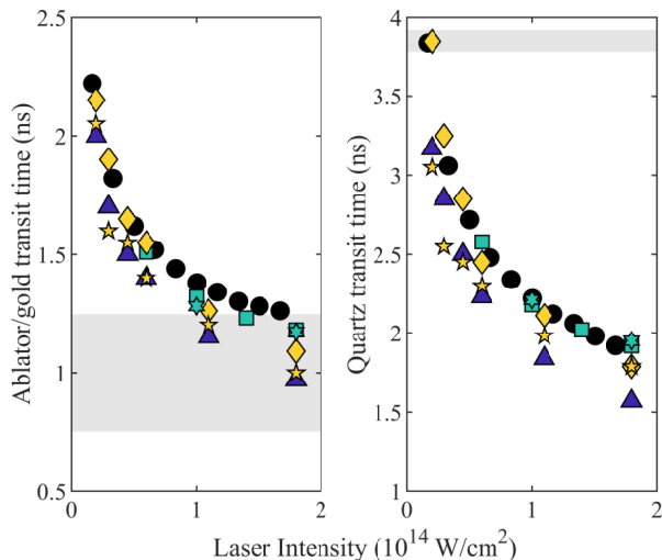
FIG. 12. Simulated shock transit times through the combined ablator/gold layers (left) and the quartz layer (right) for one of the experimental shots. This was performed in 4 different 1D radiation hydrodynamics codes: HYADES (black circles), FLASH (teal squares), MULTI (yellow diamonds) and HELIOS (blue triangles). 2D simulations were also performed in MULTI (yellow stars) and FLASH (teal hexagrams). On each plot, the grey shaded region corresponds to the experimentally measured value (bounded by the uncertainty). The agreement between codes is good, and in all cases it is not possible to match the experimentally measured times in both ablator/gold and quartz layers at any one intensity.
