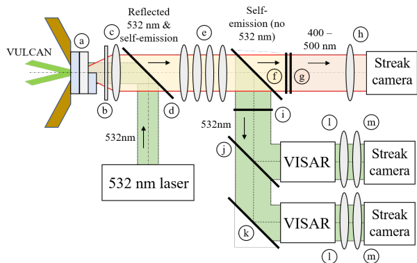
FIG. 1. A simplified schematic of the experiment. The route of different frequencies are indicated, while key components are labelled. A 532 nm laser is passed through a beamsplitter (d) through the objective lens ((c), protected by a blast shield (b)) onto the target ((a), as detailed in Figure 2). The reflected 532 nm light and self-emission is collected by the objective lens, and passes through a system of 4 lenses (e), with focal lengths of 700, 500, 700 and 250 mm. A dichroic mirror (f) separates a narrow band of wavelengths around 532 nm from the transmitted light. Filters (g) leave only the 400 - 500 nm light, which is focussed by a f = 300 mm lens (h) into a streak camera, forming the SOP system. The 532 nm is further isolated by a notch filter (i), removing any 527 nm noise from VULCAN. A beamsplitter (j) directs the light into two VISAR systems, with different etalon lengths. (k) is a simple turning mirror. Finally, a f = 300 mm lens (l) focuses the light from each of these into a separate streak camera, while a f = 200 mm cylindrical lens (m) focuses it further in the dimension perpendicular to the streak camera slit to improve signal strength. The schematic is not to scale, and additional components (such as turning mirrors) have not been displayed.
