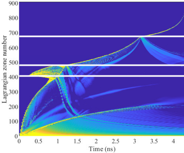
FIG. 13. Shock propagation plot (log derivative of pressure) from a 1D Helios simulation of the same shot and laser intensity as in Figure 14. It can be seen that a second shock (originating from the gold layer) catches and overtakes the primary shock just before it reaches the foam layer (this is different to the FLASH simulation, where this occurs at an earlier time). The figure is plotted as a function of Lagrangian simulation zone number (rather than radius), so that the zone material boundaries are stationary and the shock propagation can be seen more easily. The zone boundaries are indicated by the white horizontal lines.
