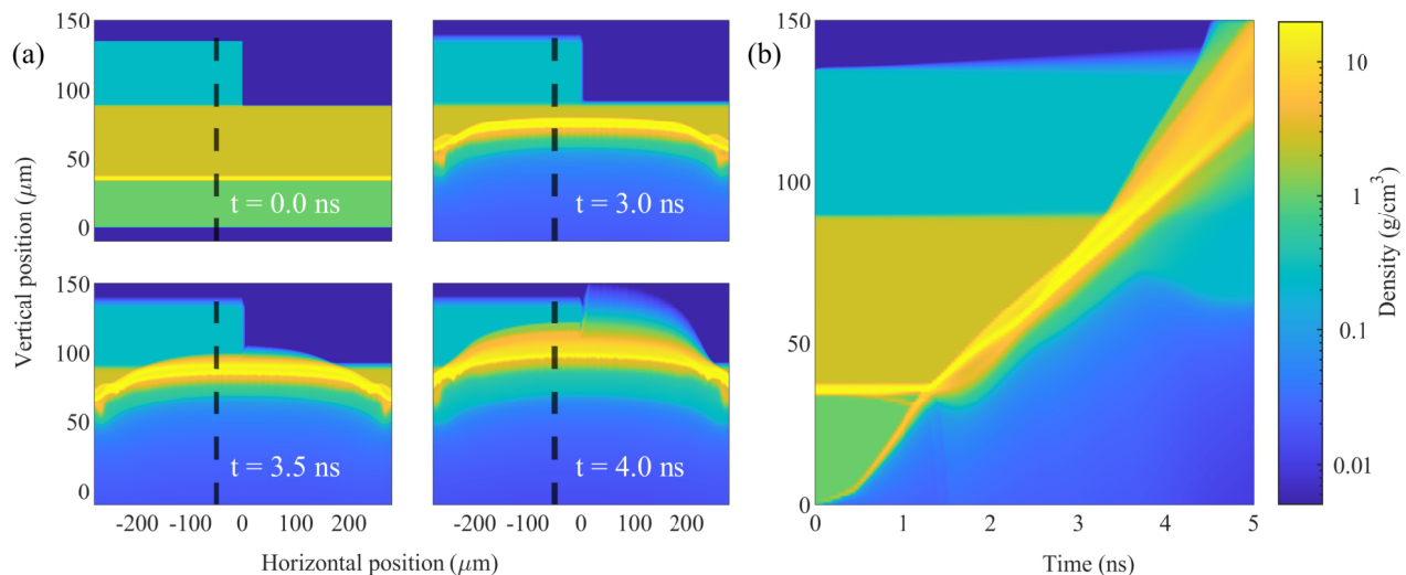
FIG. 11. 2D FLASH simulation using measured target dimensions and temporal laser profile, with a peak laser intensity of 1.8 \times 10^{14} W/cm 2 . (a) shows four snapshots of the shock propagating through the target in 2D. It can be seen that the shock propagation through the foam is largely undisturbed by the step structure. (b) shows the shock propagation vs time at a single horizontal position (50 \mu m within the target, indicated by the dashed black line in (a)). The same colour scale (representing density) is used in all plots.
