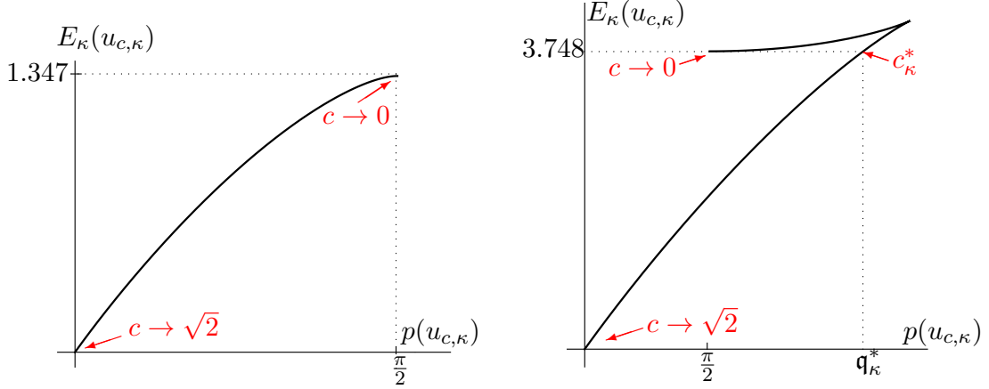
Figure 6: Energy-momentum diagram of dark solitons with parameters in \mathcal{D}_2 , with \kappa = -3 (left) and \kappa = -50 (right).
