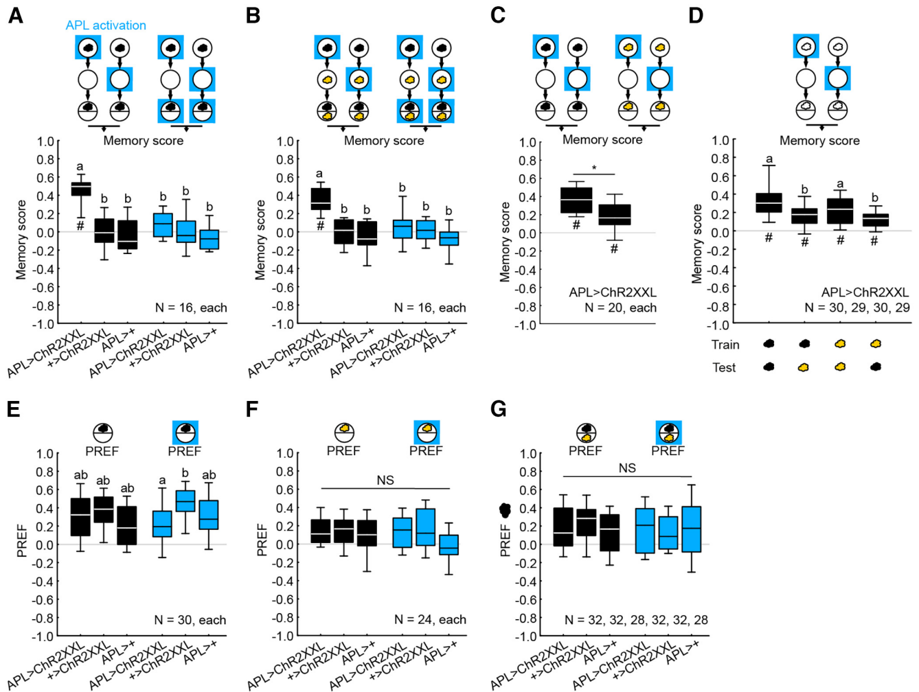
Figure 14. Activation of APL during testing prevents the behavioral expression of appetitive odor-APL memory. A , Repetition of the experiment from Figure 12A, confirming that APL activation has a rewarding effect (black-filled box plots). Activating APL during testing as well prevented the behavioral expression of appetitive odor-APL memory (blue-filled box plots). B , Larvae were trained and tested as in A , except that in a differential conditioning protocol, OCT was used as a second odor (yellow cloud) in all training trials in which AM (black cloud) was not presented. Presenting one of the two odors paired with APL activation induced odor-specific appetitive memory; as in A , testing the animals while activating APL prevented the behavioral expression of memory. C , Larvae were trained and tested as in Figure 12A either with AM (black cloud) or OCT (yellow cloud) as a single odor. Compared with AM, larvae showed lower appetitive memory scores when OCT was used as a conditioned stimulus. D , Larvae were trained as in C and tested either with the same trained odor (AM or OCT), or with the respective other novel odor (AM or OCT). Testing larvae with the novel odor led to generalization decrement. E , The behavior of experimentally naive larvae toward AM (black cloud) was tested either without APL activation or with APL activation during the test. Naive odor preference in the experimental group was unaffected by APL activation (APL>Chr2XXL) (see also Fig. 9D), with the caveat that it did differ from the effector (+>Chr2XXL), but not from the driver control (APL>+). F , Same as in E , except that OCT was used as a single odor (yellow cloud). Naive odor preference in the experimental group was unaffected by APL activation (APL>Chr2XXL), and did not differ from the genetic controls. G , Same as in E , F , except that OCT was used as a second odor (yellow cloud). Again, naive odor preference in the experimental group was unaffected by APL activation (APL>Chr2XXL) and did not differ from the genetic controls. The sample sizes and the genotypes are given within the figure. A–D , OSS comparisons to chance levels (i.e., to zero) with a BH correction: ^{\#}p < 0.05 . A , B , D , E , Different letters indicate significant differences between groups in MWW comparisons, also with a BH correction: p < 0.05 . C , Significant differences between groups in MWW comparisons. NS indicates the absence of significance between groups in MWW comparisons with a BH correction in F , and in KW comparisons in G (NS, p > 0.05 ). The source data and results of all statistical tests are documented in Extended Data Figure 3-1 and Table 2. Other details as in Figures 9-13.
