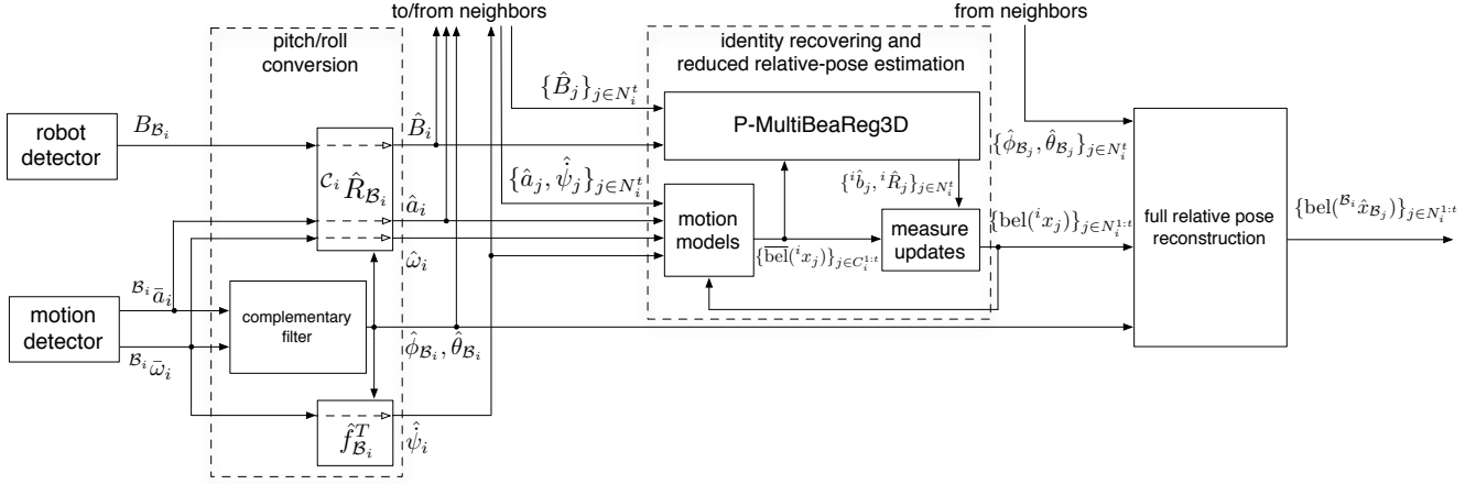
Fig. 2: Scheme of the mutual localization system that runs on the generic robot A_i .
