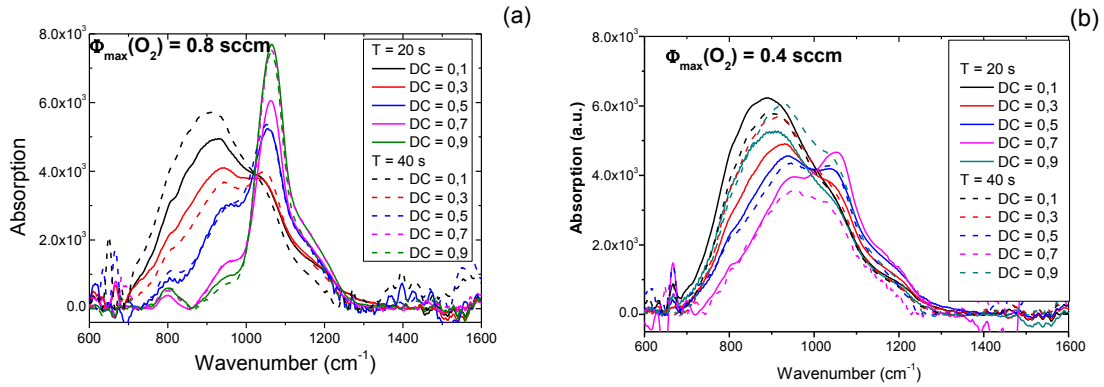
Figure 3: IR spectra for films deposited in PP with various duty cycles, for T = 20 s (full line) and T = 40 s (dash line), for (a) \Phi_{\max}(\text{O}_2) = 0.8 \text{ sccm} and (b) \Phi_{\max}(\text{O}_2) = 0.4 \text{ sccm} .
