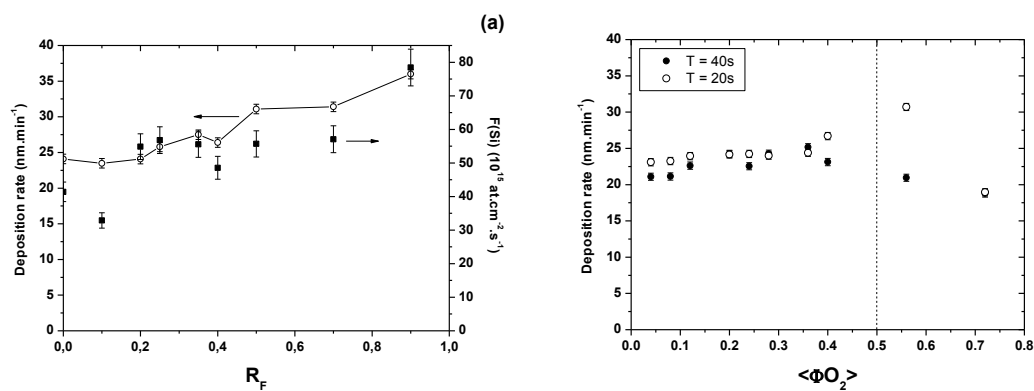
Figure 2: (a) Deposition rates (open) and incorporated silicon flux (full) calculated in CP and, (b) deposition rates in PP for both periods T = 20 (open) and 40 s (full).
