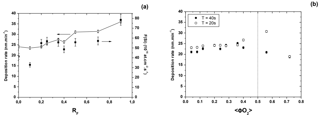
Figure 2: (a) Deposition rates (open) and incorporated silicon flux (full) calculated in CP and, (b) deposition rates in PP for both periods T = 20 (open) and 40 \text{ s} (full).
