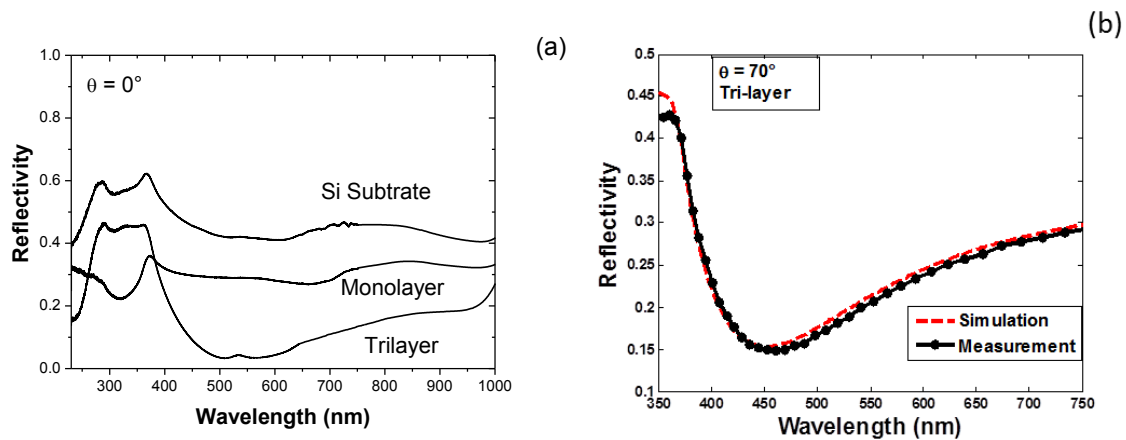
Figure 8: (a) Measured reflectivity for a normal incidence on a bare polished silicon substrate and covered by optimized mono- and tri-layer ARC, (b) measured and simulated reflectivity for a 70^\circ incident angle.
