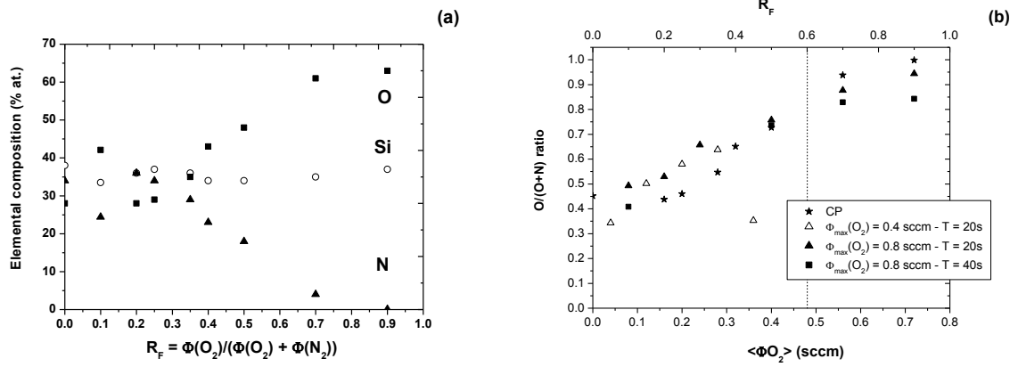
Figure 1: (a) Elemental composition of films deposited in Continuous Process and (b) O/(O+N) ratio for films deposited in continuous (star) and in pulsed process with different periods and maximum O_2 flow rates.
