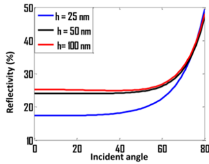
Figure 7: Simulated average reflectance as function of the incident angle for various h .
