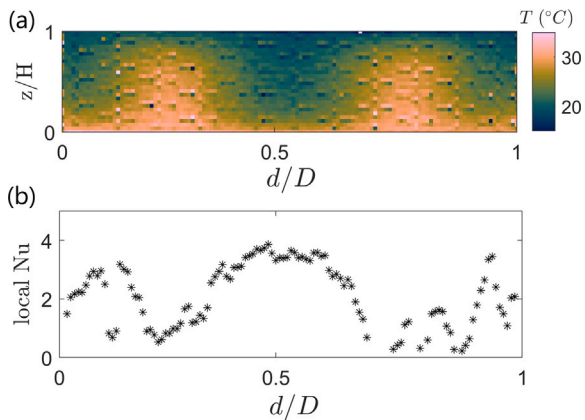
Fig. 14. Pr = 688.1 , \epsilon = 0.62 and \Delta T = 13.3 °C. (a) Measured temperature field on the xz -plane during convection. (b) Variation of the local Nusselt number along the normalized cavity's diameter d/D .
