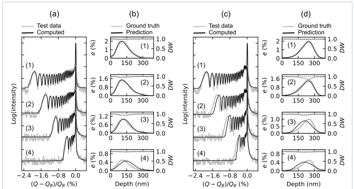
Figure 8. XRD test data (grey curves) and computed from predictions (black curves) in the case of right-hand (a) and left-hand tailed strain profiles (c). The corresponding strain profiles (grey) and DW (dotted grey) profiles are given, as well as the associated predictions (black) are given in (b), (d). The labels (1–4) correspond to decreasing maximum strain.
