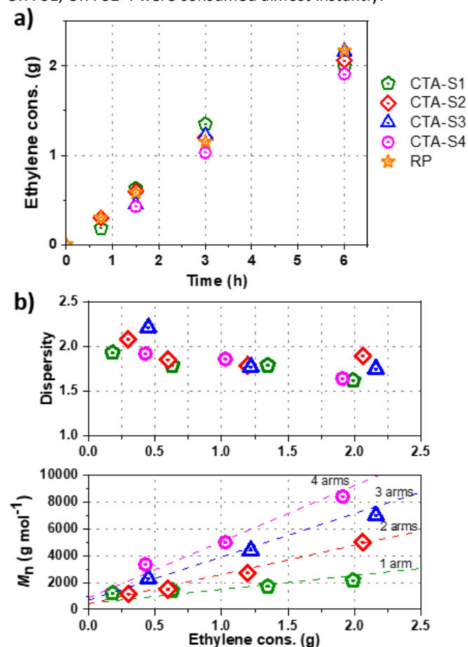
Figure 3. Polymerization conditions: T = 70 \text{ }^\circ\text{C} , P = 80 \text{ bar} , [\text{iodine}]:[\text{AIBN}] = 3:1 . Ethylene consumption = (mass of dried product) - (mass of AIBN) - (mass of CTA). a) Ethylene consumption versus polymerization time for ITP systems compared to the radical polymerization (RP) performed without CTA, and b) corresponding molar mass evolutions (from HT-SEC). Molar masses are determined by a conventional PE calibration for CTA-S1, CTA-S2 and by a universal calibration based on PS calibration for CTA-S3 and CTA-S4.
