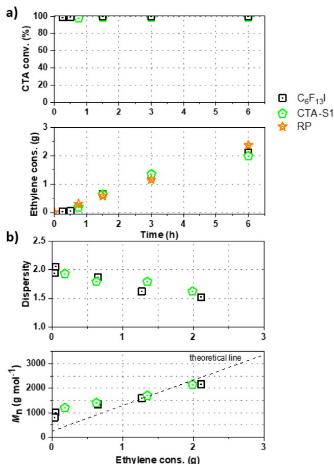
Figure 1. Polymerization conditions: T = 70\text{ }^{\circ}\text{C} , P = 80\text{ bar} , [\text{CTA}]:[\text{AIBN}] = 3:1 . Ethylene consumption = (mass of dried product) - (mass of AIBN) - (mass of CTA). a) Ethylene consumption and CTA conversion versus polymerization time for ITP systems compared to the radical polymerization (RP) performed without CTA, and b) corresponding molar mass evolutions (from HT-SEC). The radical polymerization yielded PE with M_n values of about 8000\text{ g mol}^{-1} and \bar{D} values between 1.5 and 2.1. Molar masses are determined using a conventional PE calibration.
