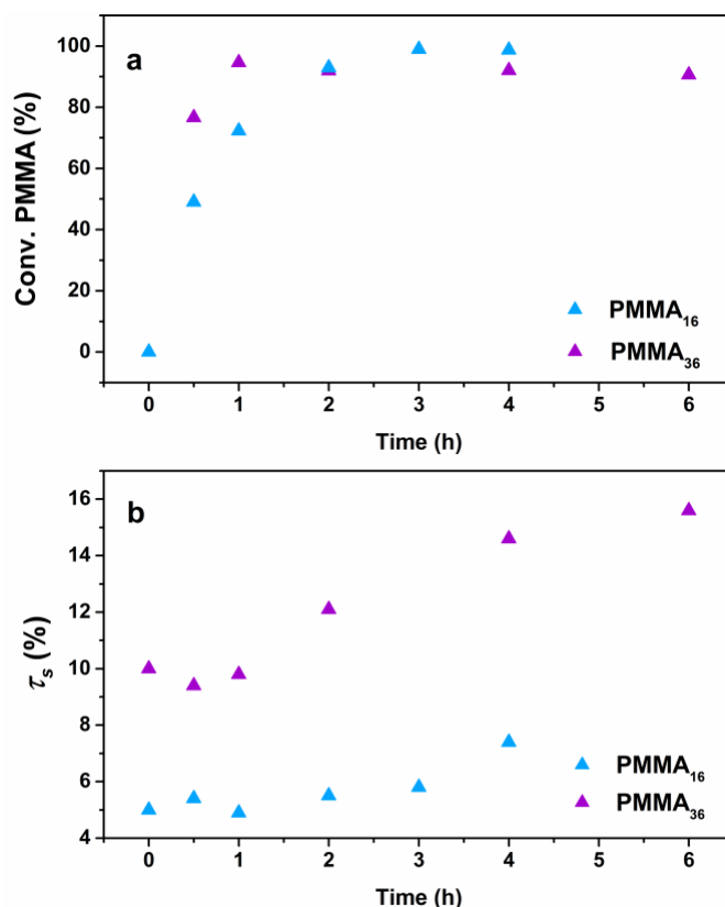
Figure 5. Evolution of a) PMMA n conversion and b) solids content with polymerization time at 80 °C and 100 bar of ethylene pressure (respectively runs 3 and 4, Table 2).
