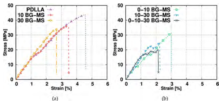
Figure 9. Stress–Strain of BG-MS 3D-printed FGM composites in (a) strategy I and (b) strategy II and III systems.
