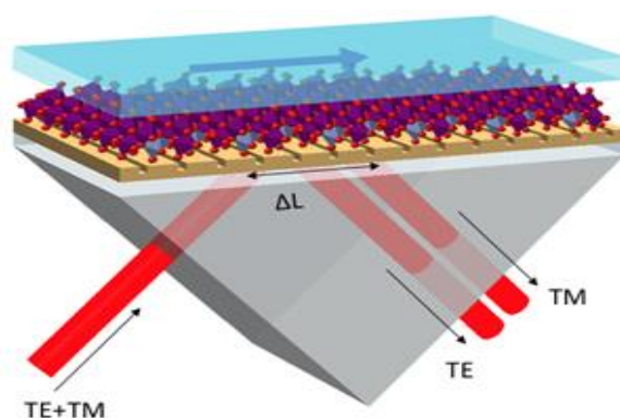
Figure 1. Schematic representing the Kretschmann SPR sensor based on a gold metasurface: prism, glass substrate, gold, and Vanadium dioxide as the sensing layer.
