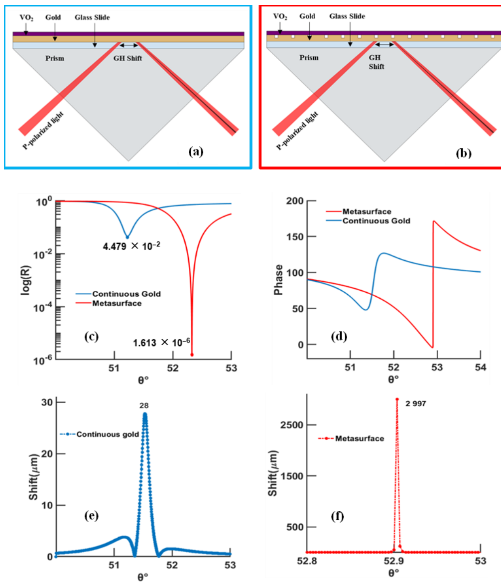
Figure 7. SPR curves calculated by TMM model, comparing the continuous gold configuration and the one with a metasurface, for an excitation of 1000 nm and VO 2 at 20°. The continuous gold thickness is equal to 50 nm, while the metasurface case includes a continuous gold layer of 30 nm and nanostructures at 20 nm depth; (a) schematic of the continuous gold configuration, (b) schematic of the metasurface configuration, (c) reflectivity, (d) phase, (e) Goos–Hänchen shift of continuous gold film (absolute value), and (f) Goos–Hänchen shift of gold metasurface (absolute value).
