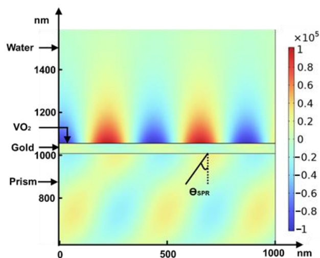
Figure 5. Electric field (y component in V/m) distribution inside the structure, given that the thicknesses of the gold film and VO 2 are 47 and 1 nm, respectively, excitation is 630 nm, and temperature is 20 °C.
