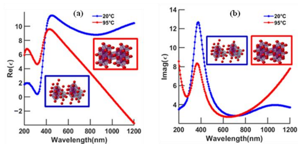
Figure 2. Experimental dielectric function: (a) real part and (b) imaginary part of VO 2 at 20 °C and 95 °C.
