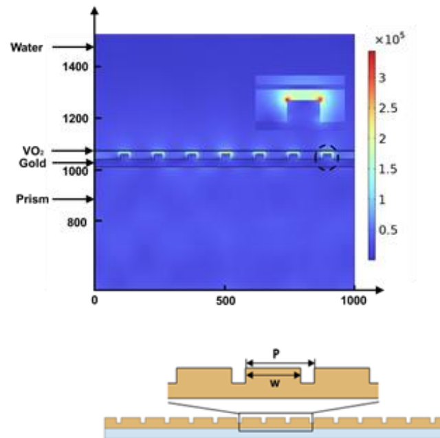
Figure 6. Electric field (norm in V/m) distribution inside the structure, given that the thickness of the continuous gold film, metasurface, and VO 2 are 30, 20, and 4 nm, respectively, for excitation 630 nm, temperature 95 °C, periodicity 130 nm, and width 30 nm.
