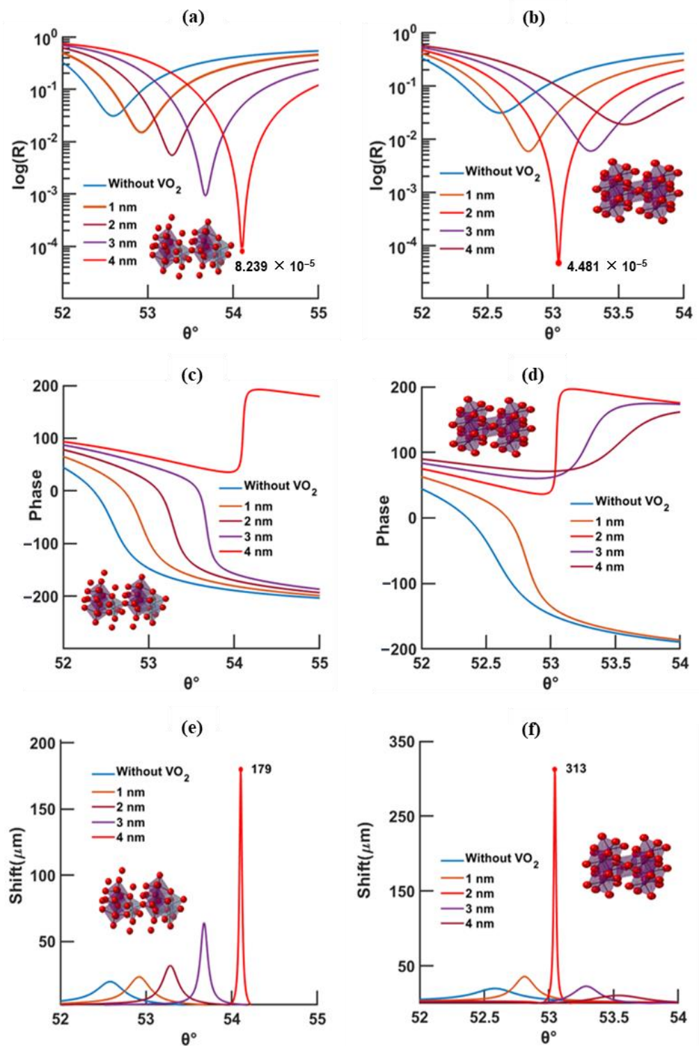
Figure 4. SPR curves with respect to the thickness of VO 2 calculated by TMM model, for an excitation of 785 nm, VO 2 temperature of 20 °C (left) and 95 °C (right), and a gold thickness of 46 nm; (a,b) reflectivity, (c,d) phase, and (e,f) Goos–Hänchen shift (absolute value).
