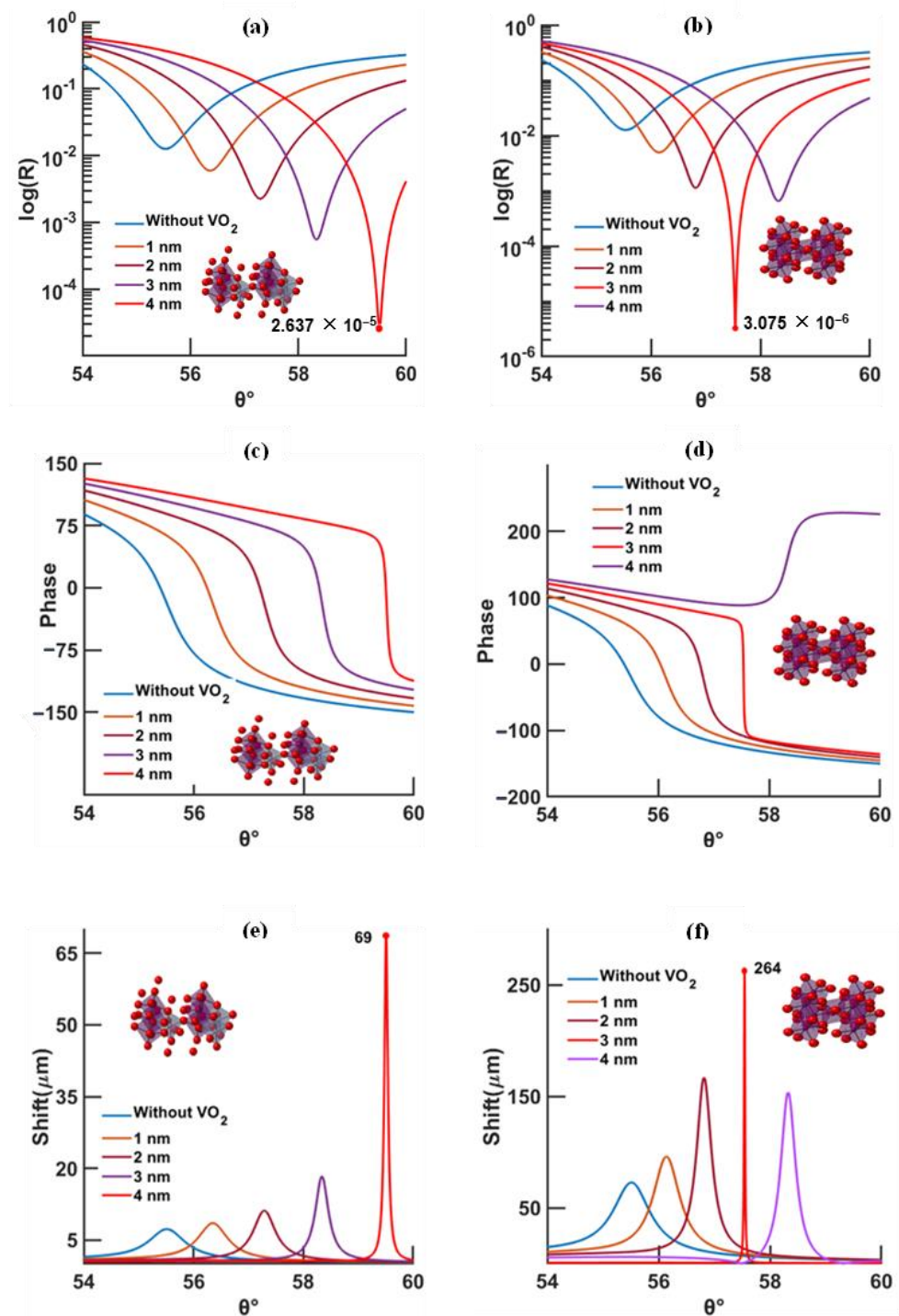
Figure 3. SPR curves with respect to the thickness of VO 2 calculated by TMM model, for an excitation of 630 nm, VO 2 temperature of 20 °C (left) and 95 °C (right), and a gold thickness of 46 nm; (a,b) reflectivity, (c,d) phase, and (e,f) Goos–Hänchen shift (absolute value).
