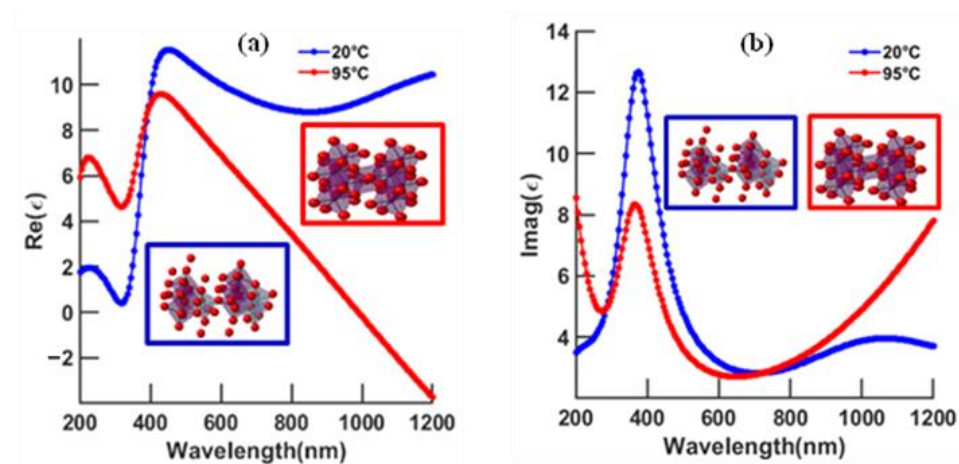
Figure 2. Experimental dielectric function: (a) real part and (b) imaginary part of VO 2 at 20 °C and 95 °C.
