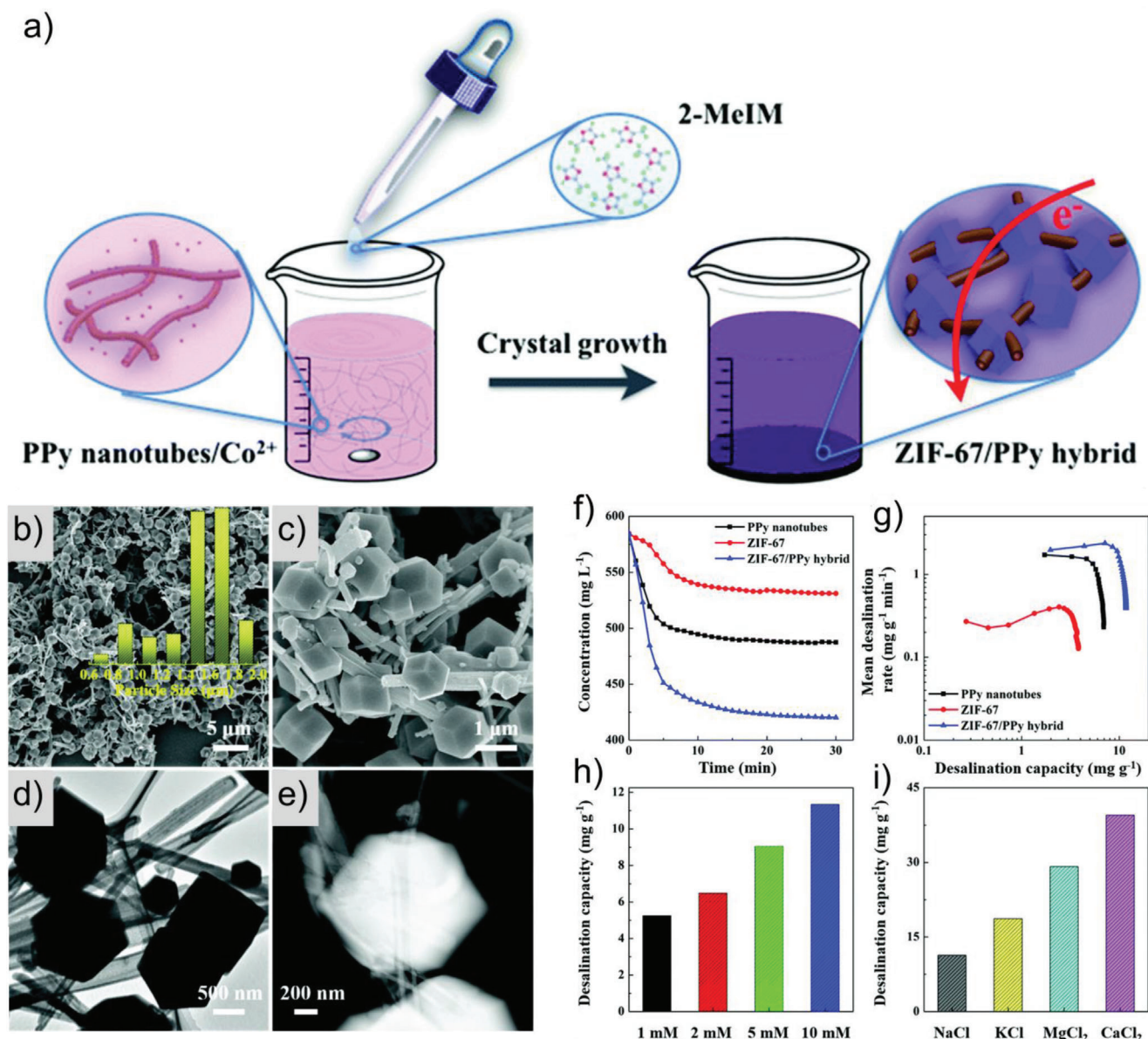
Figure 9. a) Scheme illustrating the synthetic procedure of a ZIF-67/PPy hybrid. b,c) FESEM, d) TEM, and e) HAADF-STEM images of the ZIF-67/PPy hybrid. f) Salt concentration variations and g) capacitive deionization Ragone plots of the PPy nanotubes, ZIF-67, and ZIF-67/PPy hybrid. Capacitive deionization performances of the ZIF-67/PPy hybrid h) at various NaCl concentrations and i) in various metal ion solutions (10 mM). Reproduced with permission. [188] Copyright 2019, The Royal Society of Chemistry.
