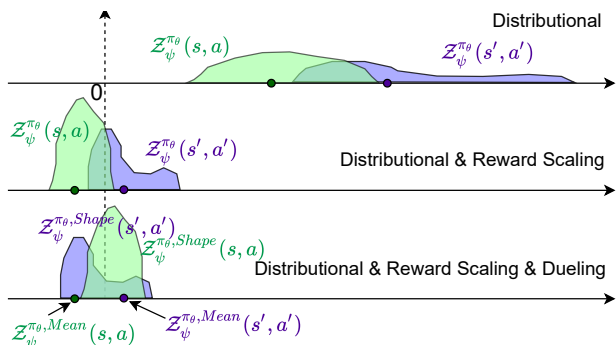
Figure 5: Effect of adding the dueling architecture in the Value Network and/or reward scaling to distributional DDPG RL.
