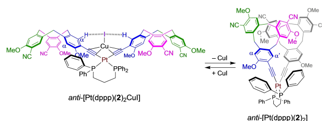
Scheme 2. Illustration, for anti -[Pt(dppp)(2) 2 ], of the chemical processes taking place at the platinum-bridged CTB dimers and the resulting conformational changes.
