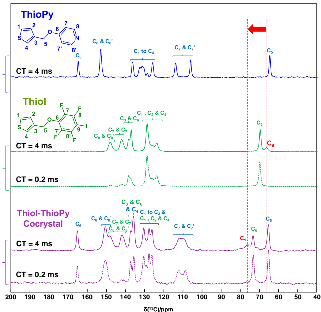
Figure 7. ^{13}\text{C} solid state NMR spectra of ThioPy (blue), ThioI (green), and the ThioI-ThioPy cocrystal (purple), recorded using cross-polarization magic-angle spinning (CPMAS) and different contact times (CT), and showing the shift in the C-I resonance ( \text{C}_9 ) upon formation of the halogen bonded cocrystal.
