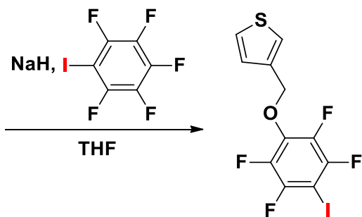
Thiol
