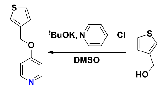
ThioPy
