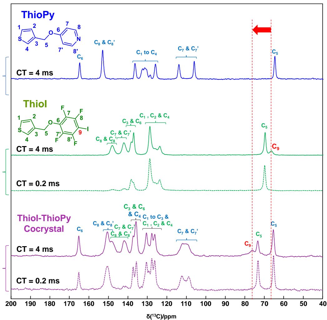
Figure 7. ^{13}\text{C} solid state NMR spectra of ThioPy (blue), ThioI (green), and the ThioI-ThioPy cocrystal (purple), recorded using cross-polarization magic-angle spinning (CPMAS) and different contact times (CT), and showing the shift in the C-I resonance ( \text{C}_9 ) upon formation of the halogen bonded cocrystal.
