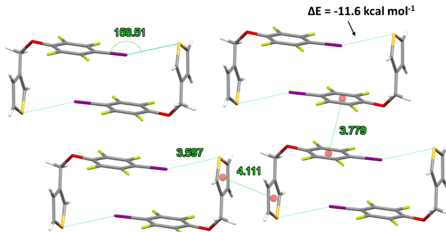
Figure 1. Packing arrangement in the X-ray structure of ThioI at 175 K developing circular motifs due to S \cdots I halogen bonds. The red dots represent the centroid of the aromatic rings. Colors are as follows: C, grey; H, white; F, yellow; S, orange; O, red; I, purple. Minor components of disordered thiophene rings in ThioI have been omitted for clarity.
