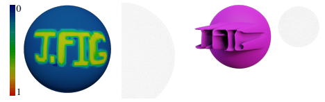
Figure 7: Weights manually painted by the user (left), and corresponding weighted elongated in-between generated with the stylization function \mathcal{S}_{\text{painted}} for a simple 3D translation (right).
