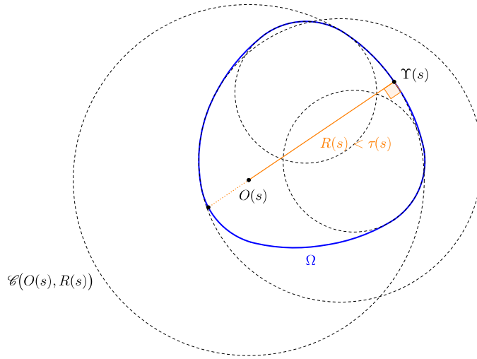
Figure 3: The geometric condition \max_{s \in \mathbb{T}} \tau(s)\mathcal{K}(s) < -1 in Definition D. Here, R(s) := -\frac{1}{\mathcal{K}(s)} is the radius of curvature, and \mathcal{C}(O(s), R(s)) is the osculating circle at \Upsilon(s) .
