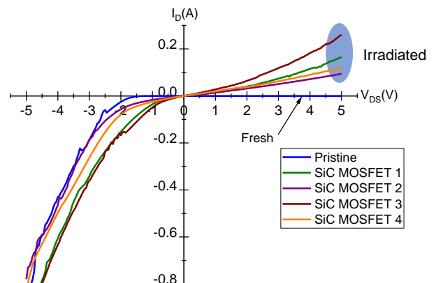
Figure 3: I_D - V_{DS} characteristics of the irradiated and failed devices. Characteristic are compared with a fresh device.
