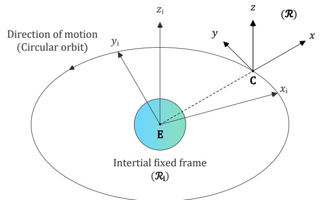
Figure 1 – Clohessy-Wiltshire frame.
