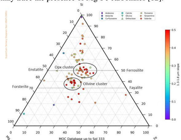
Figure 1: Si-Fe-Mg ternary diagram representing the magnitude of the 1.3 – 1.8 \mu\text{m} slope that concentrates in two clusters, one close to orthopyroxenes (Si 50 -Fe 25 -Mg 25 ) and one close to olivine (Si 40 -Fe 25 -Mg 35 ).
