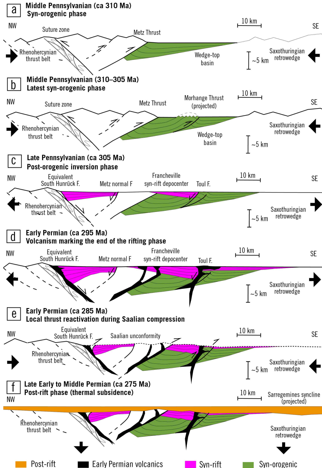
Figure 10. Schematic NW-SE cross-sections illustrating the proposed evolutionary model of the Permo-Carboniferous Lorraine Basin subdivided into 6 stages: (a) syn-orogenic basin development (Westphalian C presented here; i.e., Middle Pennsylvanian); (b) propagation of SE-verging thrusts and associated folding during Westphalian D (late Middle Pennsylvanian); (c) Post-orogenic negative tectonic inversion controlling the development of syn-rift depocenters (Stephanian/Late Pennsylvanian to Early Permian); (d) Early Permian syn-rift volcanism; (e) Local thrust reactivation during the Saalian compressional phase; (f) Post-rift thermal subsidence during late Early to Middle Permian times.
